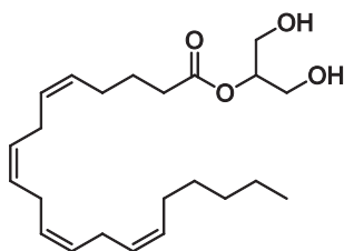
2-AG cLogP: 6.21
