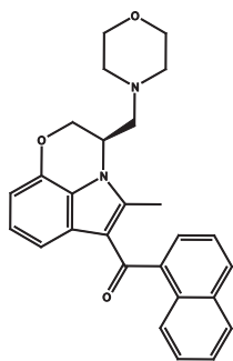
WIN55,212-2 cLogP: 4.43
