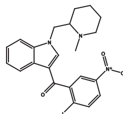
AM1241 cLogP: 3.08
