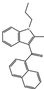
JWH015 cLogP: 5.26
