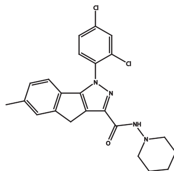
GP1a cLogP: 3.96
