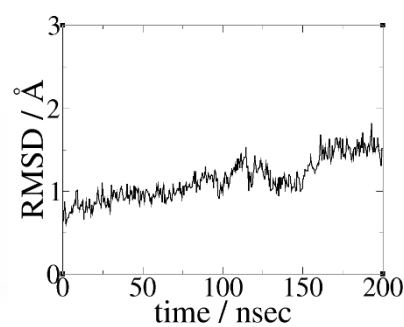
(b) docking pose8
