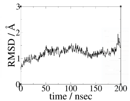
(c) docking pose6
