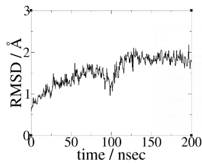
(b) docking pose5
