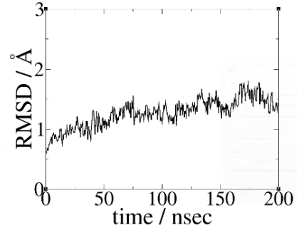
(c) docking pose3
