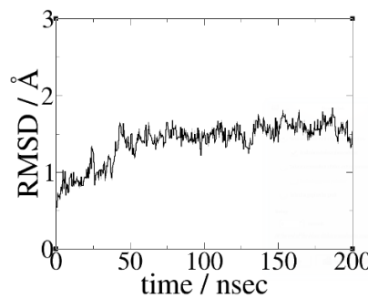
(a) docking pose7
