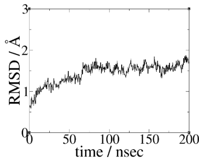
(a) docking pose4
