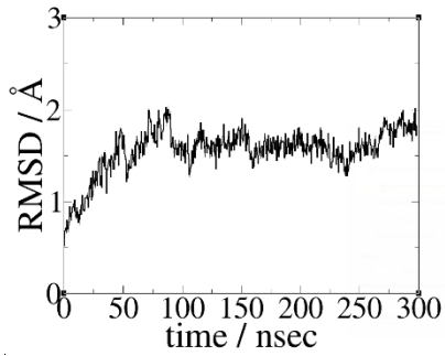
(a) docking pose1
