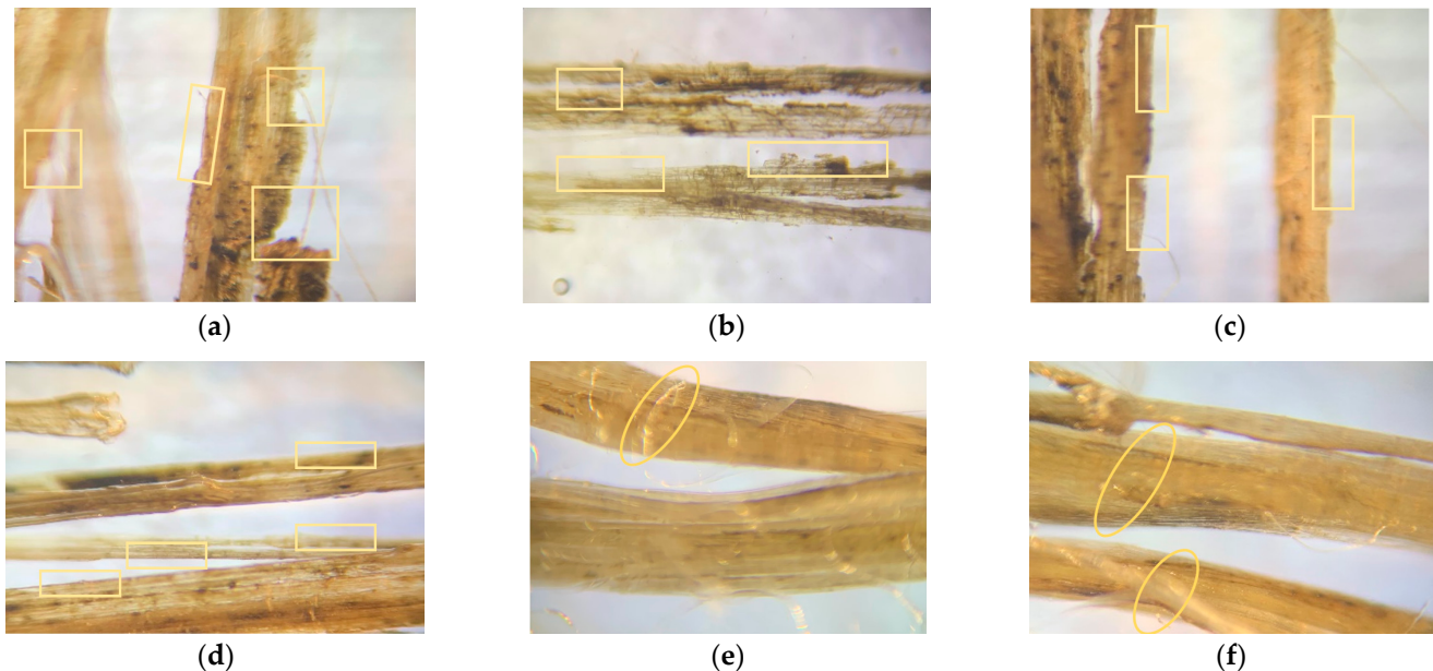
Figure 11. Microscopic images for untreated noil hemp (a), noil flax (b) fibers with microcracks, treated noil hemp (c), noil flax (d) fibers without microcracks, untreated noil hemp (e) with kink band-treated noil hemp, and (f) without kink bands.
