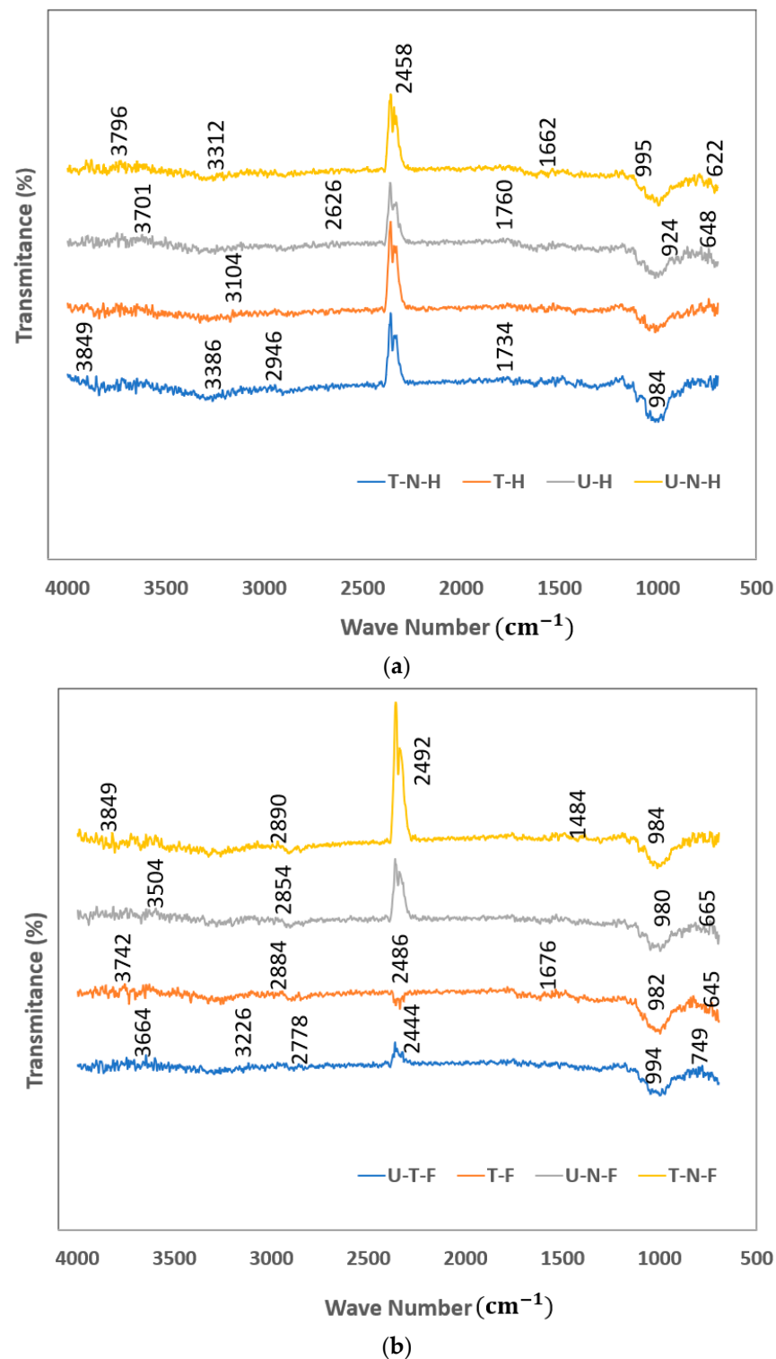
Figure 12. FTIR analysis of treated and untreated hemp and noil hemp fibers (a) and treated and untreated flax and noil flax fibers (b).
