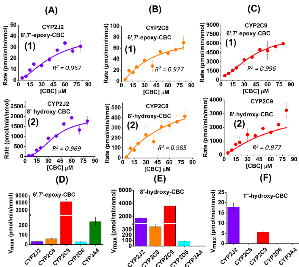
Figure 3. Metabolism of CBC by CYPs. Metabolism of CBC (0–80 μM) in the presence of CYPs leads to the formation of 6',7'-epoxy-CBC (shown in the first row as 1) and 8'-hydroxy-CBC (shown in the second row as 2) for (A) CYP2J2, (B) CYP2C8, and (C) CYP2C9. The rate of product formation is analyzed in Origin software to get the V_{\max} values. V_{\max} for (D) 6',7'-epoxy-CBC formation, (E) 8'-hydroxy-CBC formation, and (F) 1''-hydroxy-CBC formation are compared among different CYPs. Data has been fitted to either the Michaelis–Menten or Hill equation, error bars represent \pm SEM, and R^2 values for fittings are shown. (Plots for CYP2D6 and CYP3A4 are shown in the Supporting Information Figure S4 along with 1''-hydroxy-CBC formation.)
