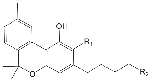
Cannabinol R_1 = H ; R_2 = CH_3 Cannabinolic acid R_1 = COOH ; R_2 = CH_3 Cannabivarin R_1 = R_2 = H
