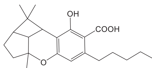
Cannabicyclic acid
