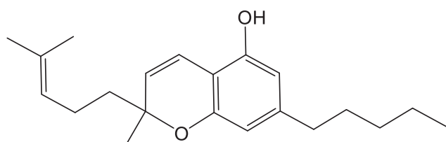
Cannabichromene
