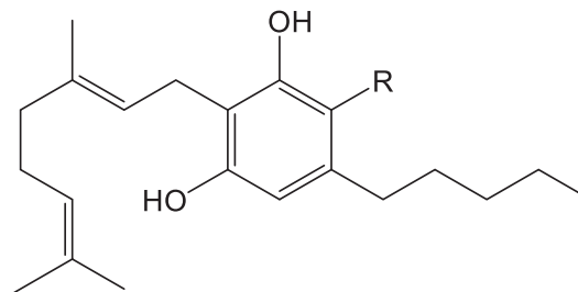
Cannabigerol R = H Cannabigerolic acid (CBGA) R = COOH
