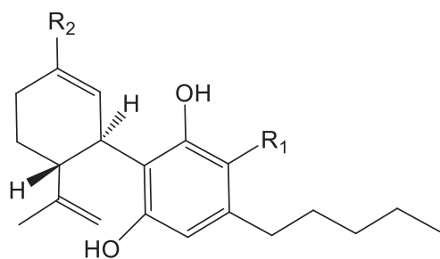
Cannabidiol (CBD) R_1 = H ; R_2 = CH_3 Cannabidiolic acid (CBDA) R_1 = COOH ; R_2 = CH_3 7-Hydroxy-cannabidiol R_1 = H ; R_2 = CH_2OH (7-Hydroxy-CBD)
