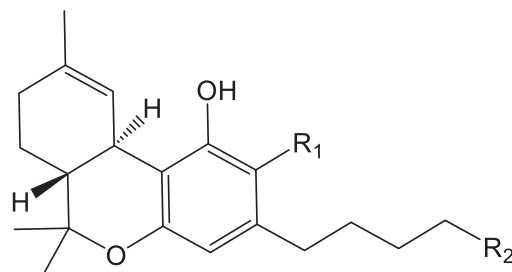
\Delta^9 -Tetrahydrocannabinol ( \Delta^9 -THC) R_1 = H ; R_2 = CH_3 \Delta^9 -Tetrahydrocannabinolic acid-A ( \Delta^9 -THCA-A) R_1 = COOH ; R_2 = CH_3 \Delta^9 -Tetrahydrocannabitol R_1 = R_2 = H
