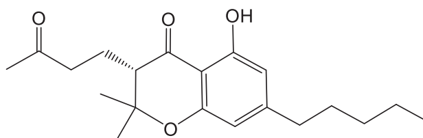
Cannabichromanon
