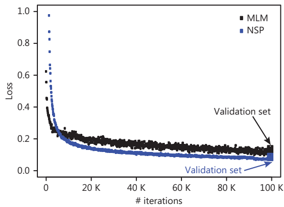
Figure S1 The loss values of the masked language model and next-sentence prediction of EhrBERT.
