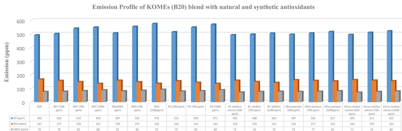
Fig. 3 Emission profile of KOMES (B20) blend with natural and synthetic antioxidants.
