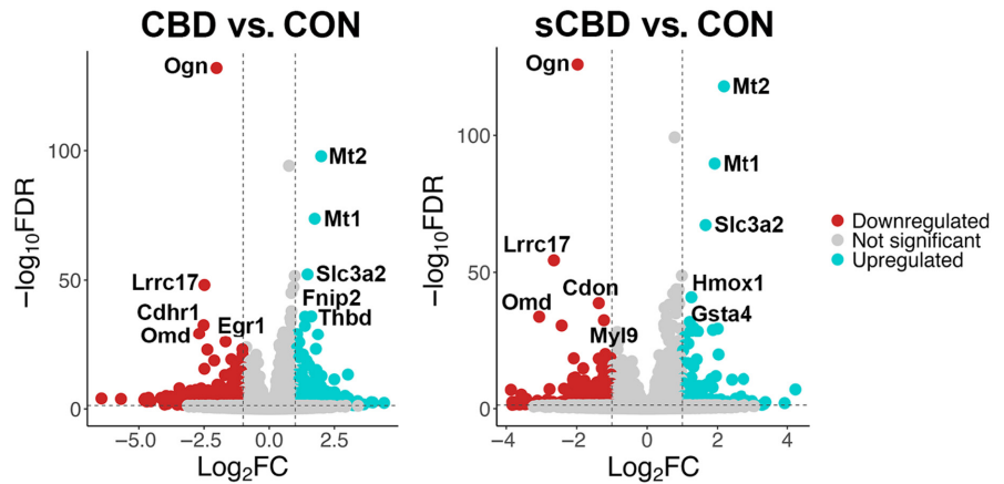
FIGURE 4 Volcano plot illustrating the relationship between -\log_{10} FDR step-up and \log_2 fold-change for DEGs. Gray data points represent genes that are not statistically significant ( -\log_{10} FDR step up < 0.05 ) and \log_2 FC > -1.1 ), whilst blue data points are significantly up regulated and red data points are significantly downregulated. Top 5 up and downregulated DEGs are labeled for comparison.
