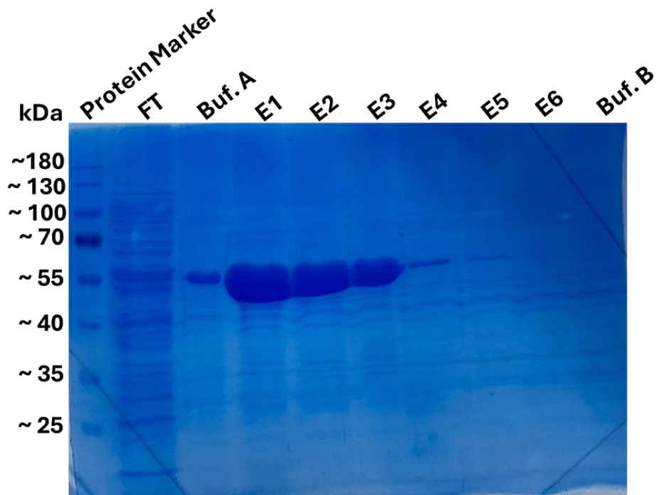
S.F.1. SDS-PAGE analysis of PmAmy after HisTrap column purification FT: Flowthrough of column passing sample; Buf. A: sodium phosphate buffer having 30 mM imidazole; E1-E2: elutions having 100, 200, and 400 mM imidazole and Buf. B: sodium phosphate buffer having 500 mM imidazole.
