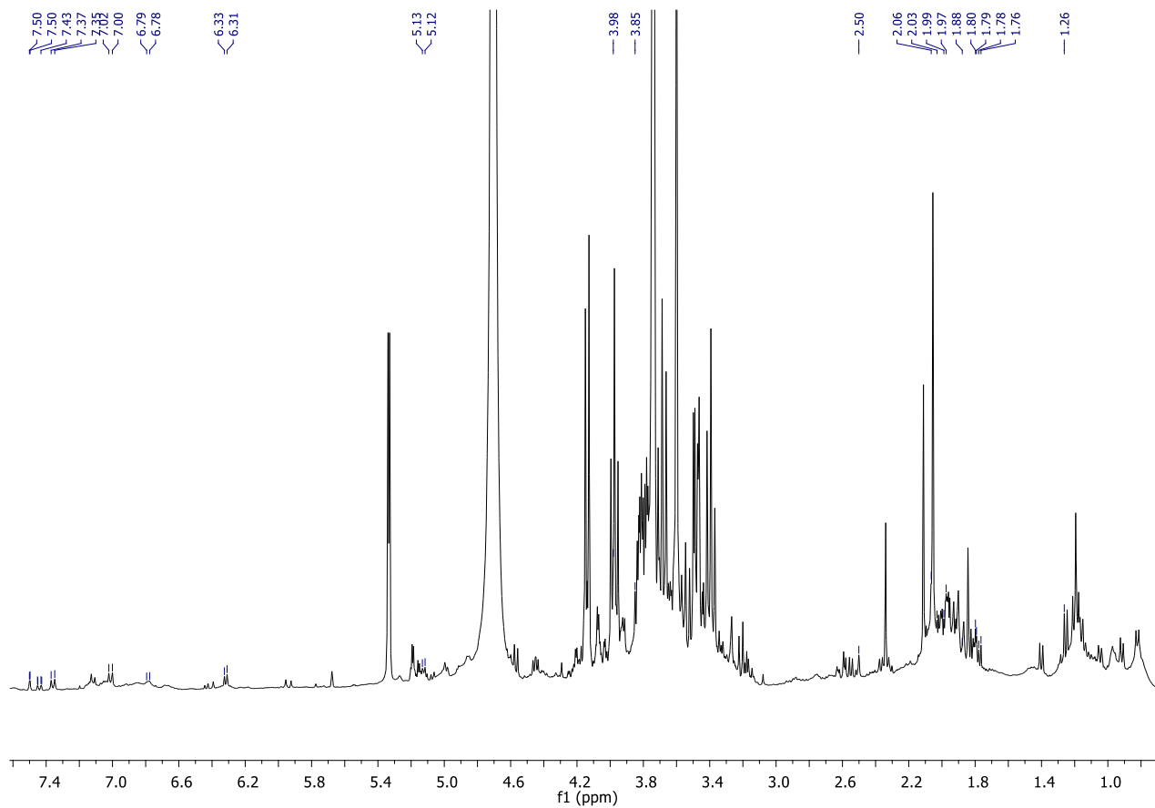
Figure S2: 1 H NMR of the assembly of fractions 34-39 from column 2
