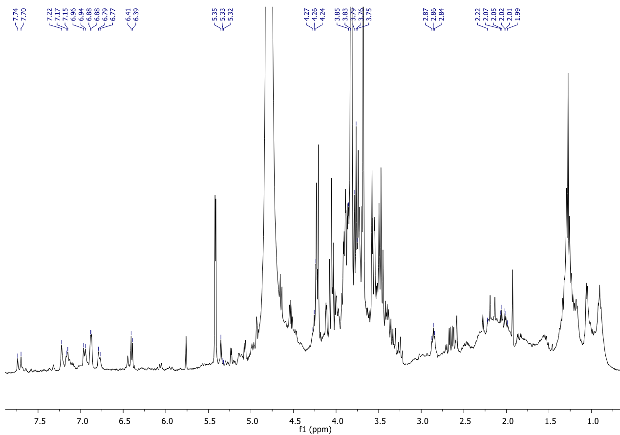
Figure S3: ^1\text{H} NMR of the column 2 methanol wash
