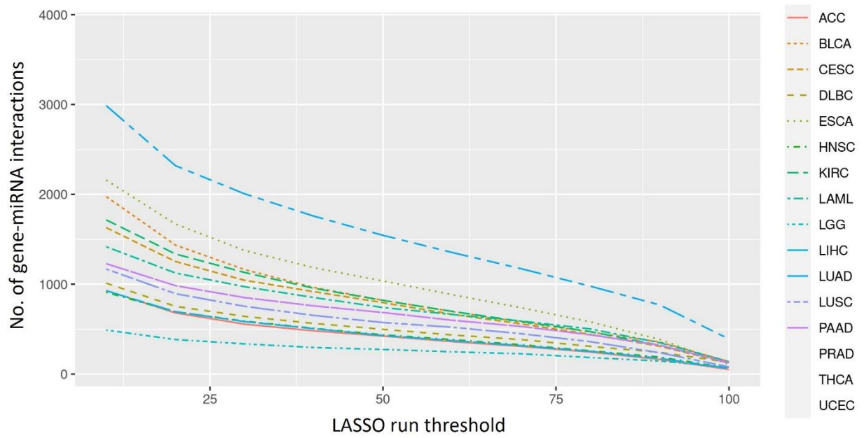
Supplemental Figure S24: Plots of the number computed miRNA-gene interactions with different LASSO runs for computing the miRNA regulators with non-zero coefficients.
