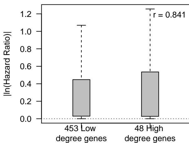
UCEC PFI
