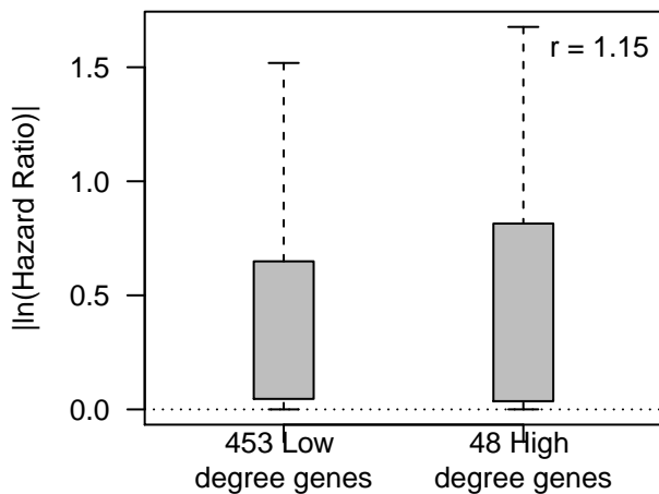
UCEC DFI
