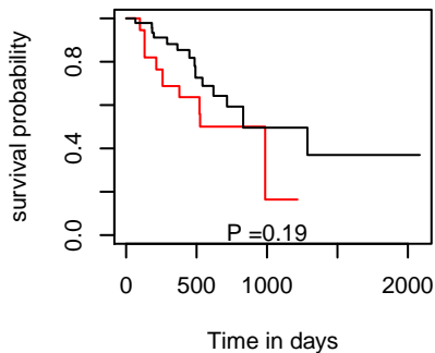
DFI hsa-mir-4763
