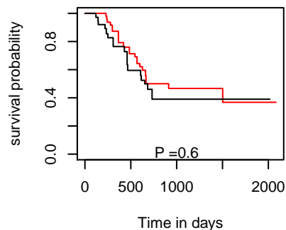
DSS hsa-mir-653
