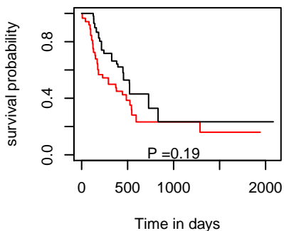
PFI hsa-mir-937
