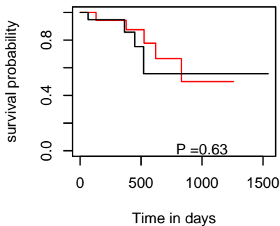
DFI hsa-mir-3648
