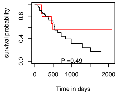
DFI hsa-mir-876
