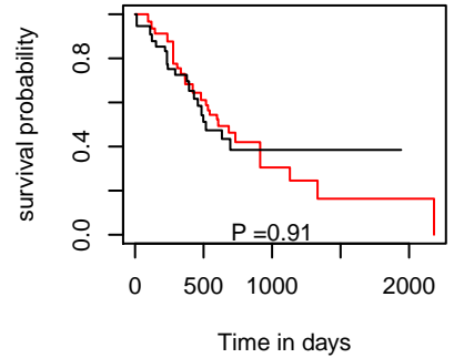
OS hsa-mir-6720
