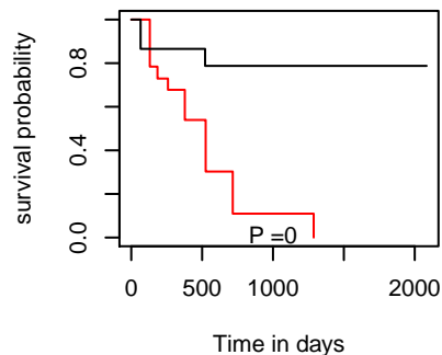
DFI hsa-mir-6510
