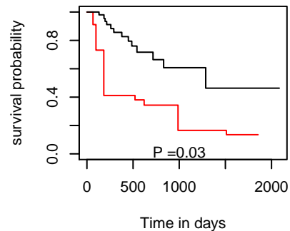
DFI hsa-mir-4687
