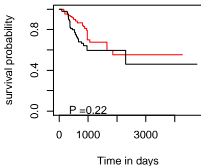
DSS hsa-mir-106b
