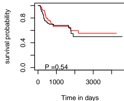
PFI hsa-mir-217
