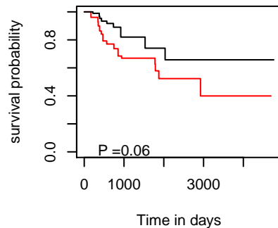
DFI hsa-mir-3607
