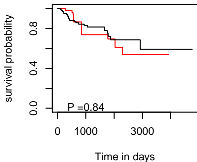
DFI hsa-mir-499a
