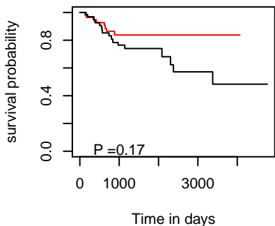
DSS hsa-mir-887
