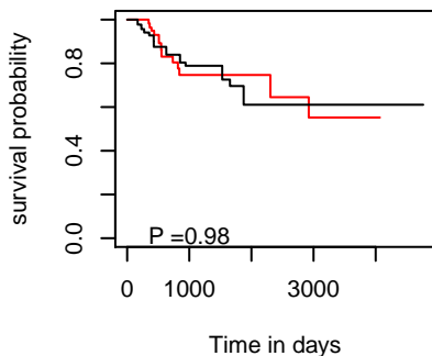
DFI hsa-mir-580
