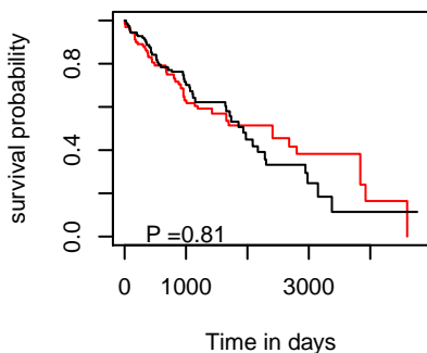
OS hsa-mir-7-2
