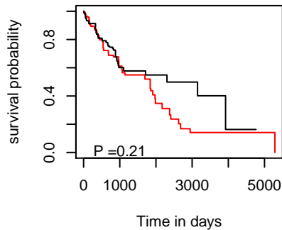
OS hsa-mir-935
