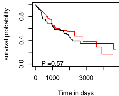
OS hsa-mir-185
