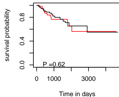
DFI hsa-mir-6803
