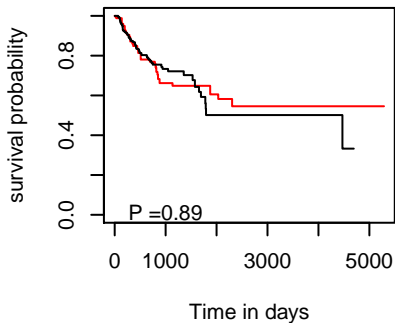
PFI hsa-mir-4707
