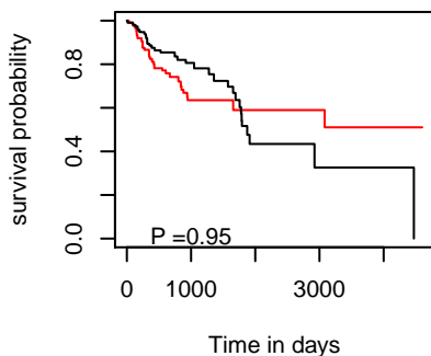
PFI hsa-mir-7-2
