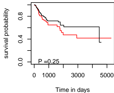
PFI hsa-mir-4645
