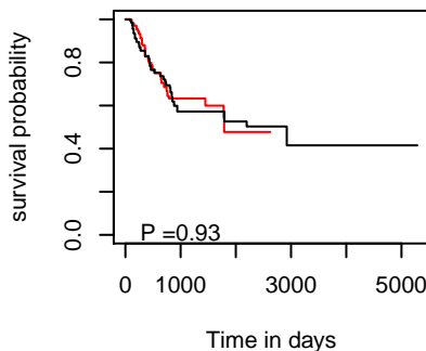
PFI hsa-mir-3926-1
