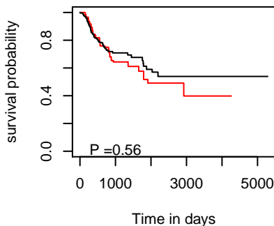
PFI hsa-mir-641
