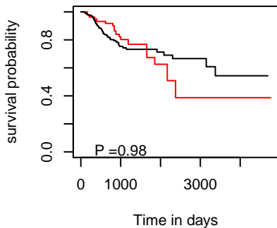
DSS hsa-mir-6851
