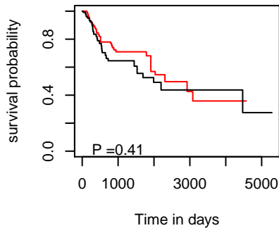
PFI hsa-mir-130b
