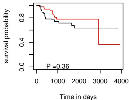
DFI hsa-mir-3682
