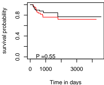
DFI hsa-mir-217
