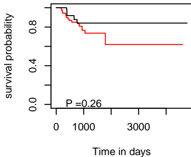
DFI hsa-mir-6511b-1
