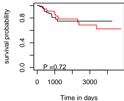
DSS hsa-let-7b
