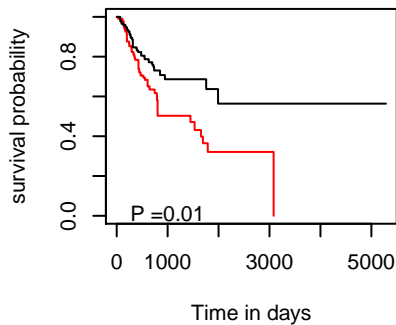
PFI hsa-mir-326
