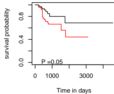
DFI hsa-mir-326
