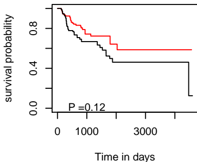
PFI hsa-mir-185
