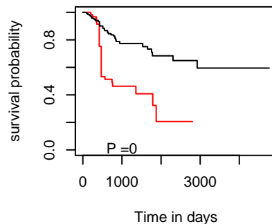
DFI hsa-mir-3667
