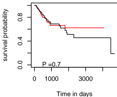
PFI hsa-mir-887
