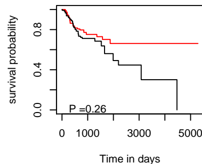
PFI hsa-mir-153-2
