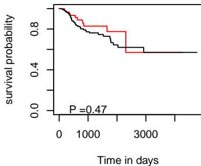
DFI hsa-mir-4286
