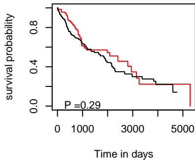
OS hsa-mir-4755
