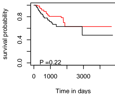
DFI hsa-mir-6802
