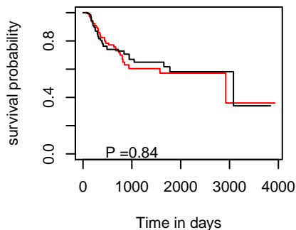
PFI hsa-mir-3682
