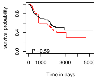
PFI hsa-mir-4492
