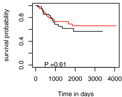
DSS hsa-mir-197
