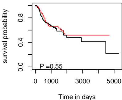
PFI hsa-mir-6802
