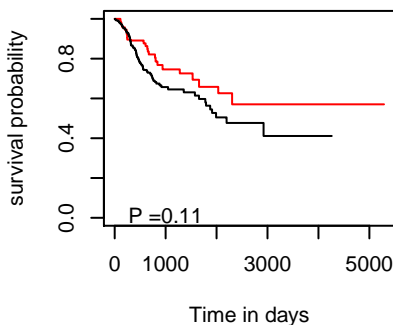
PFI hsa-mir-3618
