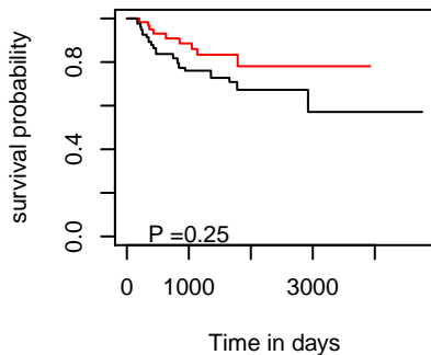
DFI hsa-mir-3691
