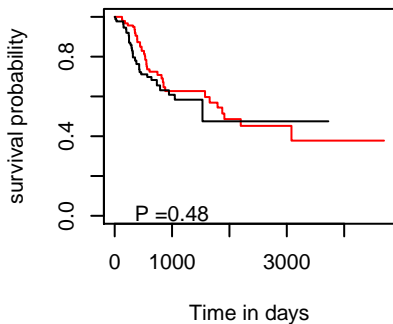
PFI hsa-mir-653
