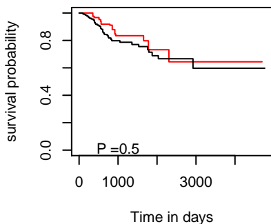
DFI hsa-mir-1275
