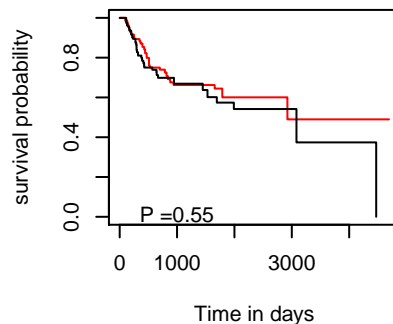
PFI hsa-mir-301b
