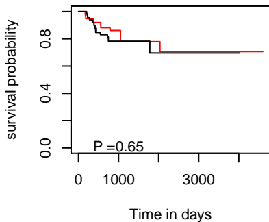
DFI hsa-mir-7704
