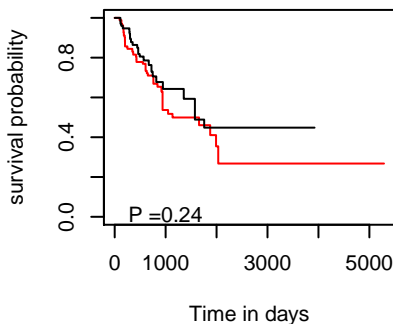
PFI hsa-mir-3934
