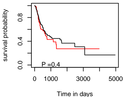
PFI hsa-mir-3176
