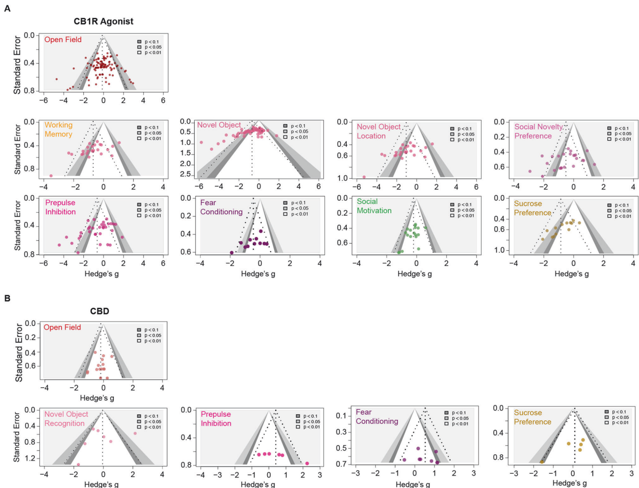
Fig. 4 Contour-enhanced funnel plots for assessing potential publication bias. In each plot, effect sizes (Hedge's g ) are plotted on the x-axis and standard errors on an inverted y-axis. Each coloured dot on the plot represents a single effect size data point. The dashed lines form an idealised funnel shape that indicates the expected distribution of studies. The vertical line in the middle of the funnel represents the average effect size. The contours from light to dark grey signify the significance levels of the data points, with darker shades representing higher significance levels ( p < 0.01 , p < 0.05 , and p < 0.1 ). A Funnel plots displaying the distribution of individual effect estimates from experiments assessing CB1R agonists effects across nine behavioural tests. B Funnel plots displaying the distribution of individual effect estimates from experiments assessing CBD effects across five behavioural tests.
