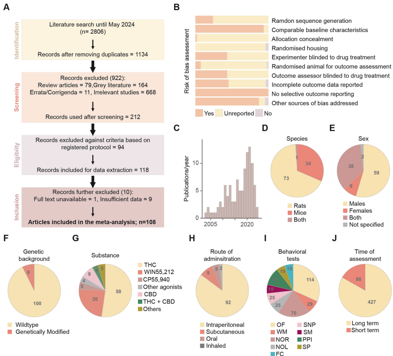
Fig. 1 Article screening and general characteristics of the studies included. A Flowchart of the screening strategy for the articles returned from electronic databases and the number of studies excluded at each step. B Cumulative bar charts displaying risk of bias assessment across 10 items specified in SYRCL's assessment tool. C Histogram showing the trend in articles published every year between 2003 and 2024 included in the meta-analysis. Pie charts depicting the proportion and number of studies categorised by species ( D ), sex ( E ), genetic background ( F ), substance administered ( G ), route of administration ( H ), the number of behavioural tests reported ( I ), and timing of behavioural tests (short term: 24 h to 10 d after final dose; long term: >10 d after final dose) ( J ). OF novelty-induced locomotion in an open field, WM working memory, NOR novel object recognition, NOL novel object location, SNP social novelty preference, PPI prepulse inhibition, FC fear conditioning, SM social motivation, SP sucrose preference.
