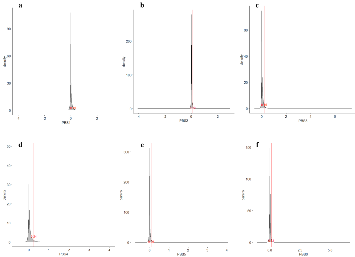
Figure S1 PBS distributions of various comparisons between populations, with the African population as the outgroup. (a) PBS1, divergence of the European population from the East Asian population; (b) PBS2, divergence of the European population from the South Asian population; (c) PBS3, divergence of the East Asian population from the South Asian population; (d) PBS4, divergence of the East Asian population from the European population; (e) PBS5, divergence of the South Asian population from the European population; (f) PBS6, divergence of the South Asian population from the East Asian population. Top 5% values were set as the thresholds.
