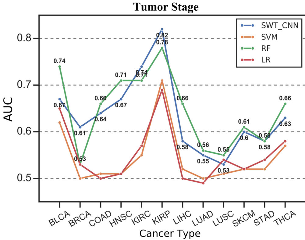
Figure 1. The performance of SWT-CNN, SVM, random forest and logistic regression on predicting the tumor stages of all cancer types.
