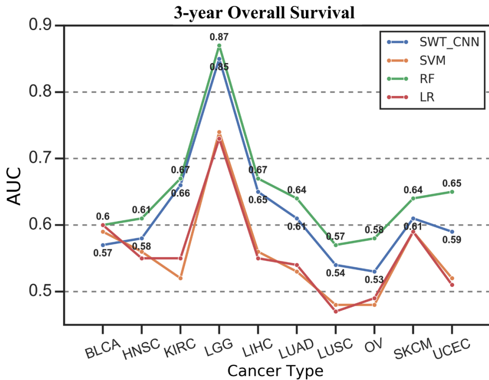
Figure 2. The performance of SWT-CNN, SVM, random forest and logistic regression on predicting the 3-year overall survivals of all cancer types.
