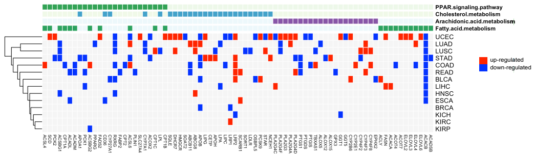
Fig. S1. Gene expression levels with mutation frequency more than 2% and differently expressed in pan-cancer. Genes with up-regulated or low-regulated in four pathways across multiple cancer types are respectively shown in red and blue ( |\log_{2}FC| > 1 , FDR < 0.05 ).
