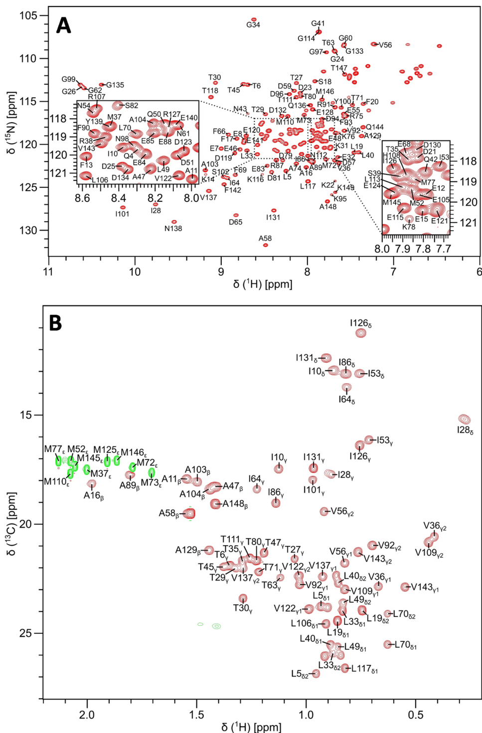
Fig. 1 Two-dimensional NMR spectra of CaM under standard conditions at neutral pH. A ^{15}\text{N} - ^1\text{H} HSQC spectrum recorded at 600 MHz ^1\text{H} frequency was analyzed to determine backbone resonance assignments. The spectrally crowded regions are highlighted with black-dashed boxes (see inset). B Constant-time ^{13}\text{C} - ^1\text{H} HSQC spectrum was analyzed to determine aliphatic side chain resonance assignments. Representative resonance assignments are indicated by residue labels; complete assignments are available as BMRB accession no. 51289
