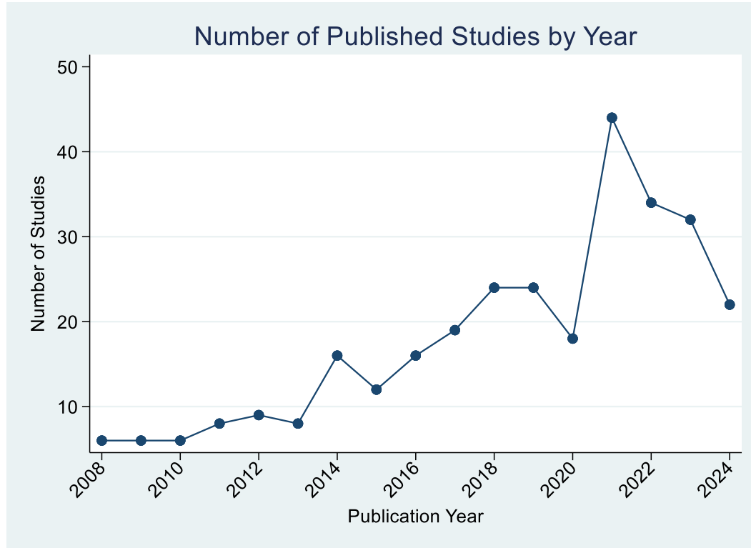
Figure S1. Number of included studies by publication year (k = 304)
