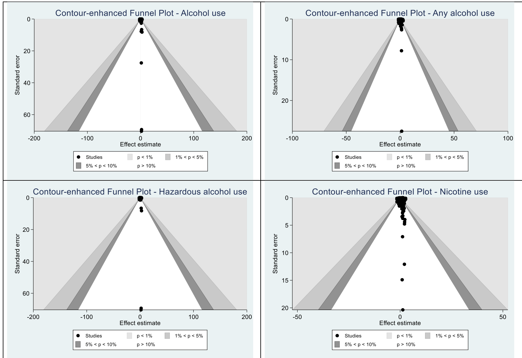
Figure S3. Contour-enhanced funnel plot for dichotomous outcomes
