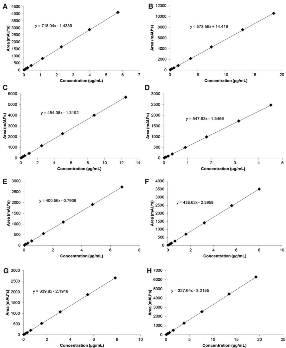
SUPPLEMENTARY FIG. S6. Calibration curve obtained for each analyte ( n=3 ). Formaldehyde ( A ), acetaldehyde ( B ), acetone ( C ), acrolein ( D ), propionaldehyde ( E ), crotonaldehyde ( F ), 2-butanone ( G ), and butyraldehyde ( H ).
