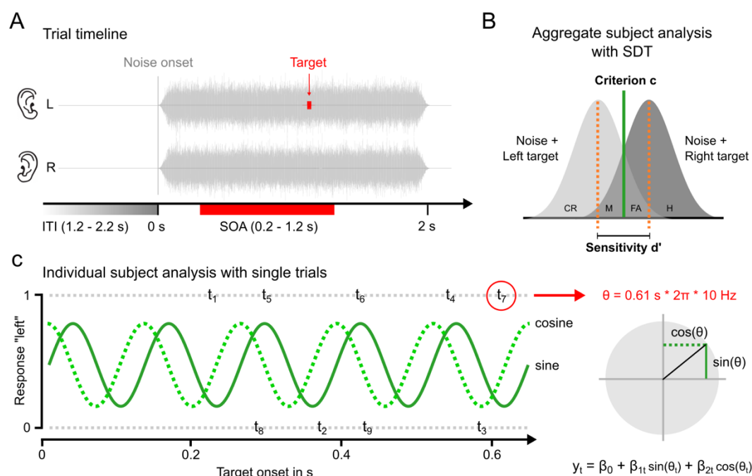
Figure 1. (A) Schematic of a trial. On each trial, white noise was presented simultaneously to both ears for 2 s. A pure tone of 1 kHz and 10 ms duration was delivered with equiprobability to the left or right ear. The SOA was randomly selected from an interval of 0.2-1.2 s post noise onset. The ITI jittered randomly between 1.2-2.2 s. (B) Application of signal detection theory (SDT). To look for oscillations in sensitivity and criterion, we first pooled across all 15 participants (creating an aggregate subject) and binned the data with non-overlapping, rectangular windows of 10 ms. For each bin, we calculated d-prime ( d' ) and decision criterion ( c ) using the hits (H) and false alarm (FA) from the left- and right-target conditions, respectively. (M: misses, CR: correct rejections). The calculations follow the Equations 1-2. (C) Schematic illustration of the linear regression analysis based on single trials. We
