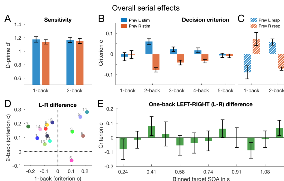
Figure 2. Results of the serial dependence analysis. (A) Group mean sensitivity contingent on whether the last (1-back) and second last (2-back) target occurred the left (blue bars) or right ear (red bars). There was no significant influence of stimulus history on observer sensitivity. (B) Group mean response bias contingent on the ear of origin of the preceding 1- to 5-back stimuli. The difference between the contingent left and right (blue and red bars, respectively) are significant for the 2-, 3- and 4-back stimuli (FDR corrected). (C) Group mean response bias contingent on the response 1-2 trials back. The difference between the contingent left and right (blue and red bars, respectively) is significant for both 1- and 2-back (FDR corrected). (D) Individual stimulus-based bias differences in the 1-back plotted against those in the 2-back. These differences were computed by subtracting the contingent left bias (blue bars in (B)) from the contingent right bias (red bars). Except for subject 5, all other subjects show a positive bias difference in the 2-back. In contrast, there was greater subject variability in the 1-back, with only 5 participants showing a positive effect. (E) Temporal dynamics of the 1-back effect. The individual response data were grouped into 12 bins of 83 ms. For each bin, we computed the difference in left and right bias contingent on the preceding trial as in (C) and averaged across all participants. Not only does the difference in bias change from negative to positive but it also increases and decreases in a smooth transition depending on the target SOA (from noise onset), suggesting that the 1-back effect fluctuates rhythmically over time. All error bars indicate \pm 1 MSE.
