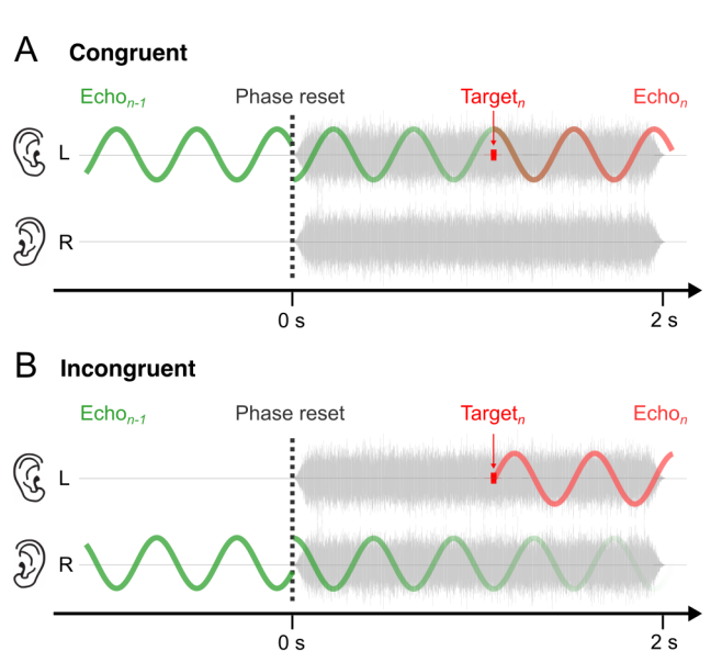
Figure 8. Possible mechanisms by which past sensory experience biases forthcoming perceptual decisions, causing oscillations in congruent but not incongruent trials. (A) The green oscillation represents the ‘echo’ evoked by a target in the left ear in the previous trial ( n-1 ). The reverberation resonates at alpha rhythm and continues to the current trial ( n ) where
