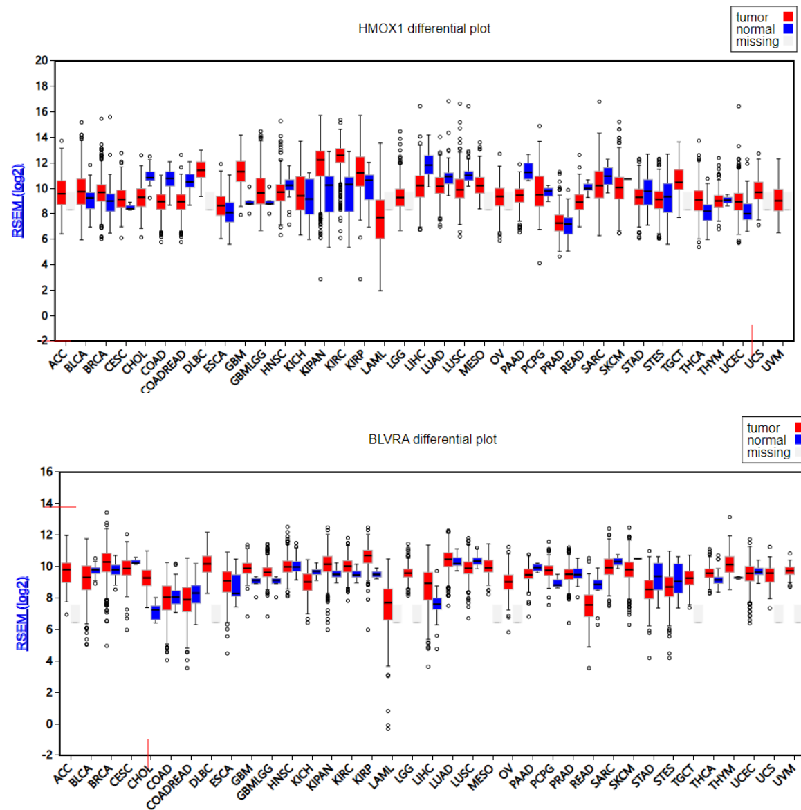
Supp Fig. 1. Expression of HMOX1 and BLVRA in various cancer tissues. (This plot was obtained from website, firebrowe.org)
