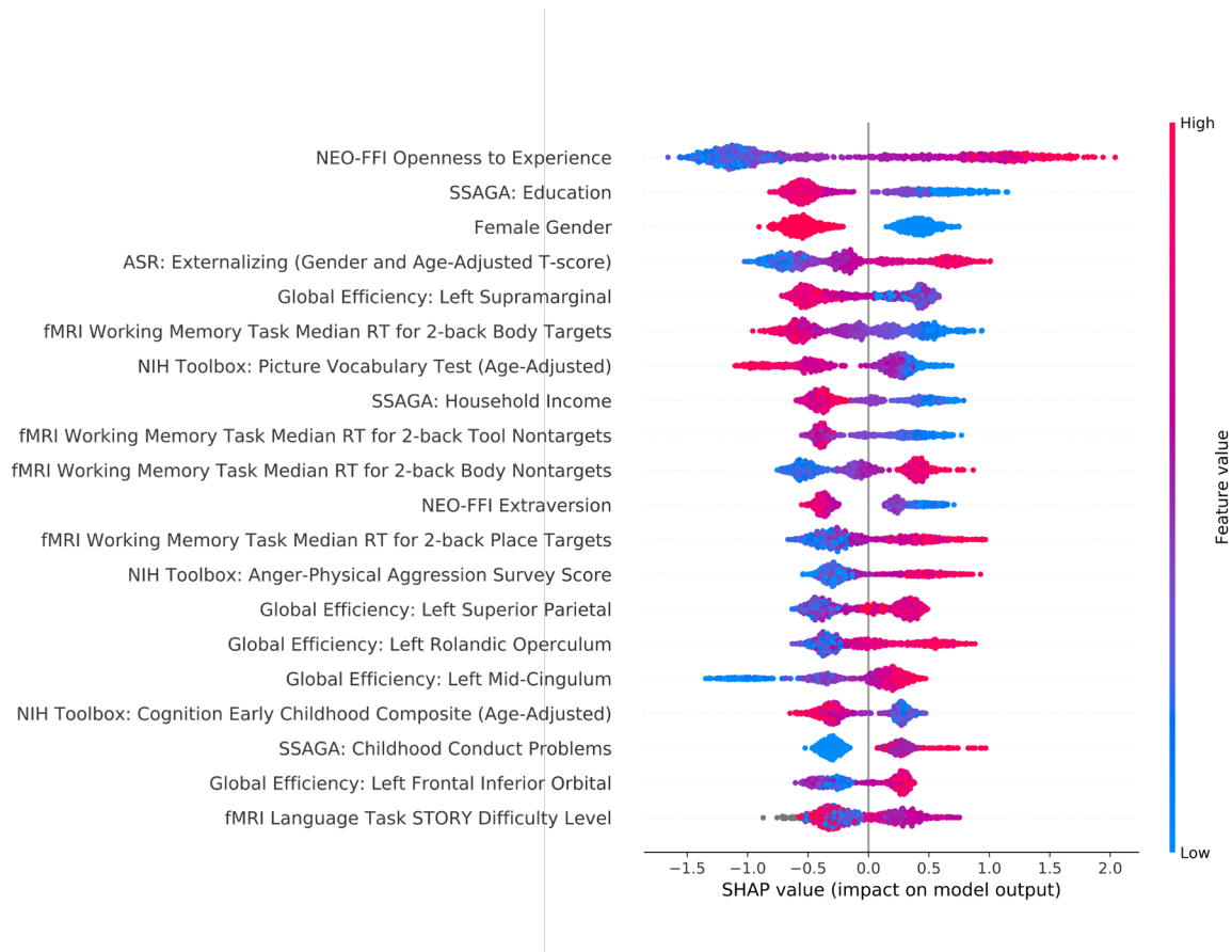
Figure S1. SHAP factor ranking for the phenotypic+Global Efficiency model classifying 100+ lifetime cannabis users. Factors are ranked in order of greatest average SHAP value, which indicates the importance of the factor. Individual points represent the model output for each individual in the sample. The position of a dot on the x-axis represents the impact of the observed factor on the model output for the individual. More positive SHAP values on the x-axis indicate that the observed factor pushed the classification closer towards cannabis dependence, whereas more negative SHAP values indicate that the factor pushed the classification away from cannabis dependence. The color of the individual dots represent the value of the observed measurements, with blue indicating lower and red higher values.
