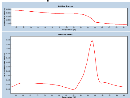
βActin
