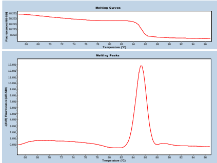
CB2R
