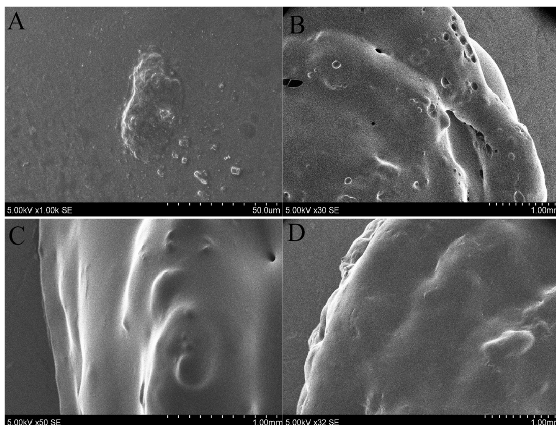
Figure 11. The visual representation via SEM analysis of the API crystals incorporated in the printlet (A), the porosity and its distribution of the experimental group gelatine–pectin printlets (B), and the visible layered structure (C,D) of the experimental group gelatine–pectin printlets.
