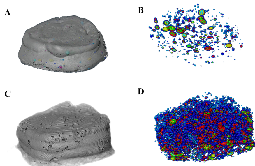
Figure 13. Visual 3D \mu -CT images of the printlets: (A) T1 gelatine–pectin control printlet external visual, (B) the distribution of voids and pores in the gelatine–pectin control printlet, (C) T2 gelatine–pectin experimental printlet external visual, (D) the distribution of voids and pores in the gelatine–pectin experimental printlet.
