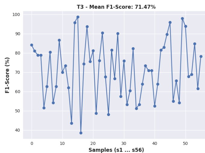
Figure 6: F1-Score percentage obtained from TP, FP, and FN considering Contact and Remote extracted peaks
