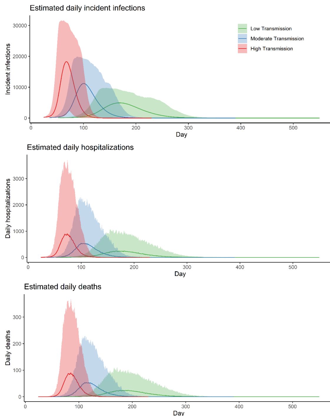
Fig 1. Simulated outbreak trajectories for Kutupalong-Balukhali Expansion Site camps under three transmission scenarios: low transmission ( R_0 = 1.5-2.0 ), moderate transmission ( R_0 = 2.0-3.0 ), and high transmission ( R_0 = 3.3-5.0 ). (A) daily incident number of people infected by COVID-19, (B) daily incident hospitalizations, and (C) daily deaths under the three scenarios. The solid lines represent the mean outbreak trajectories and the shading represents the 95% prediction intervals of each scenario.
