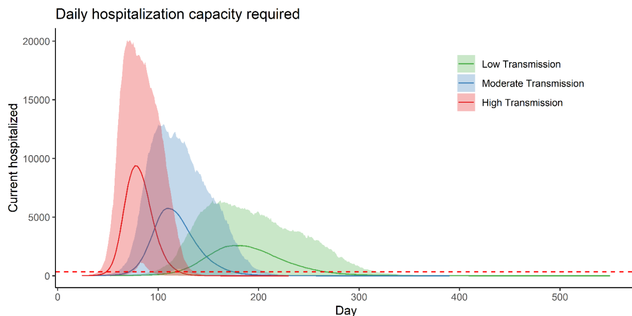
Fig 2. Hospitalization capacity requirements for an outbreak of SARS-CoV-2 in the Kutupalong-Balukhali camps, under three transmission scenarios: low transmission ( R_0=1.5-2.0 ), moderate transmission ( R_0=2.0-3.0 ), and high transmission ( R_0=3.3-5.0 ). The solid lines represent the mean outbreak trajectories and the shading represents the 95% prediction intervals of each scenario. The dashed red line represents the 340-bed surge capacity currently believed to exist in the population.
