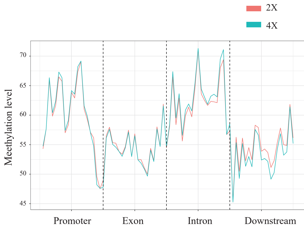
CHG gene elements profiling
