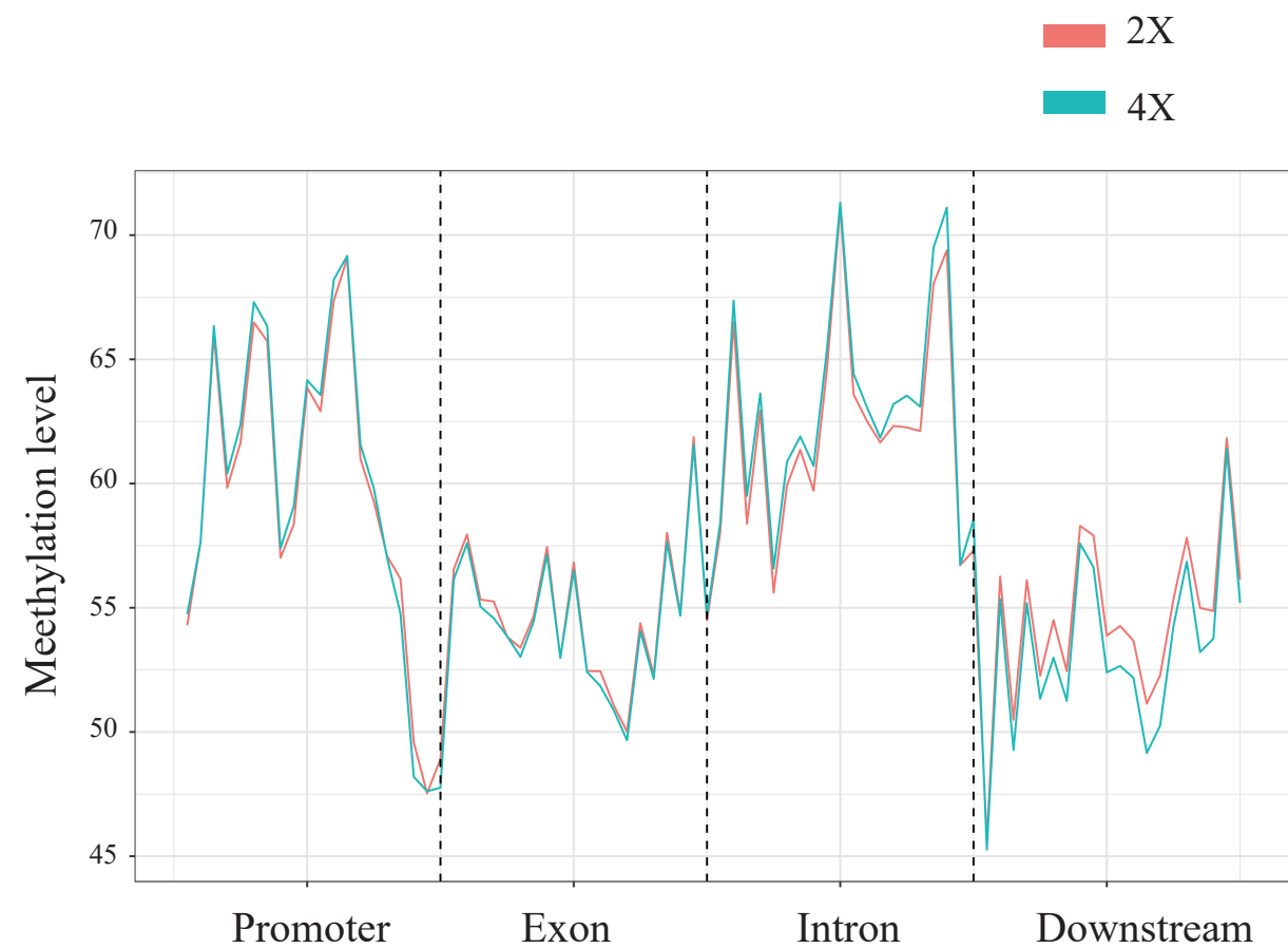
CpG gene elements profiling
