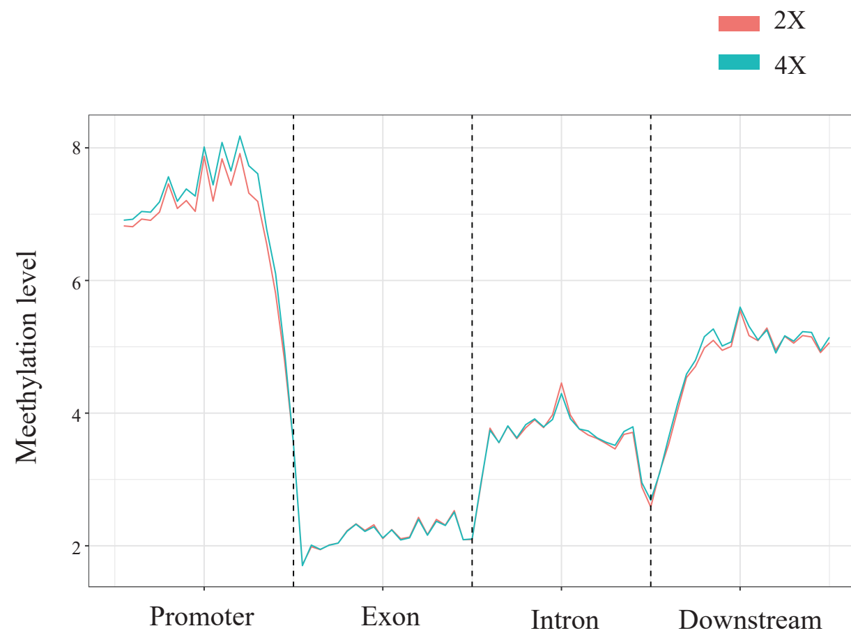
CHH gene elements profiling
