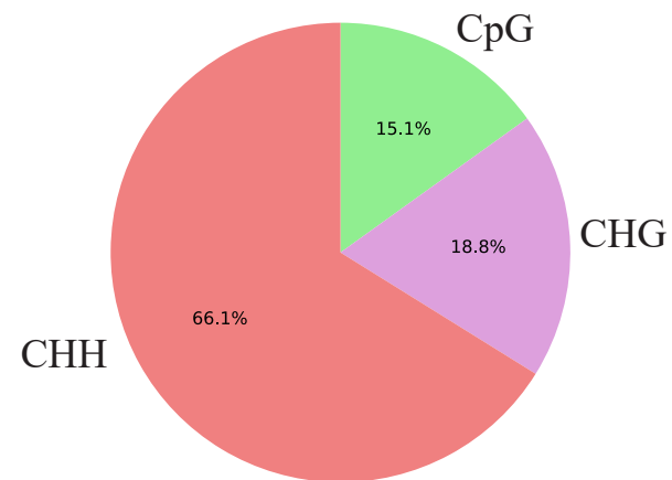
Distribution of mC types 2X
