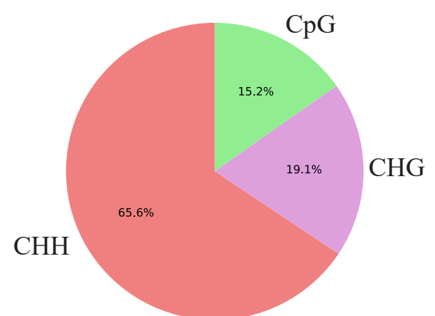
Distribution of mC types 4X
