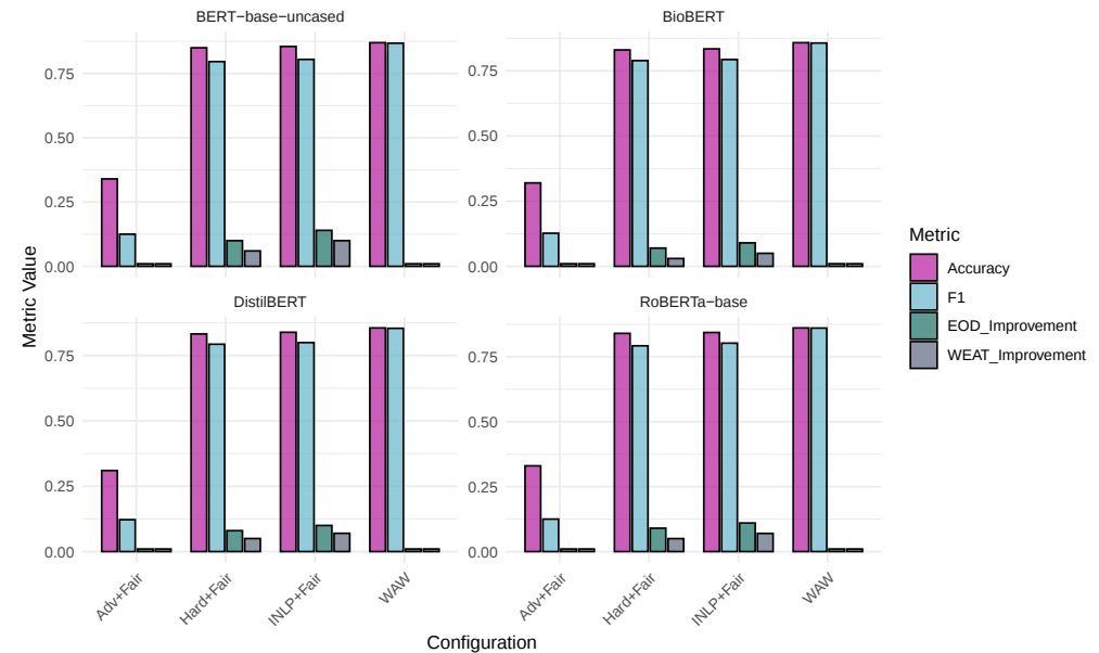
Fig 4. Comparison of BERT Models with Different Debiasing Techniques. The figure presents a comprehensive comparison of different BERT models (DistilBERT, BioBERT, RoBERTa, BERT-base-uncased) under various configurations, including no debiasing, adversarial debiasing, and fairness with projective debiasing. Metrics such as Accuracy, F1 score, Equalized Odds (EOD), and WEAT are shown. The bar charts illustrate the impact of debiasing techniques on model performance and fairness.
