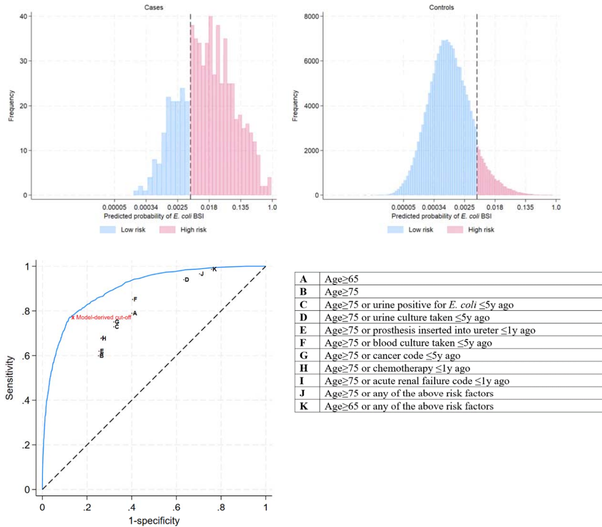
Figure 3: The predicted probability distribution in the low- and high-risk groups, as defined using the Youden index for cases (top left panel) and controls (top right panel), and Receiver Operating Characteristic (ROC) curve for the predicted probability from logistic regression model with vaccination criteria marked using letters (bottom panel).
