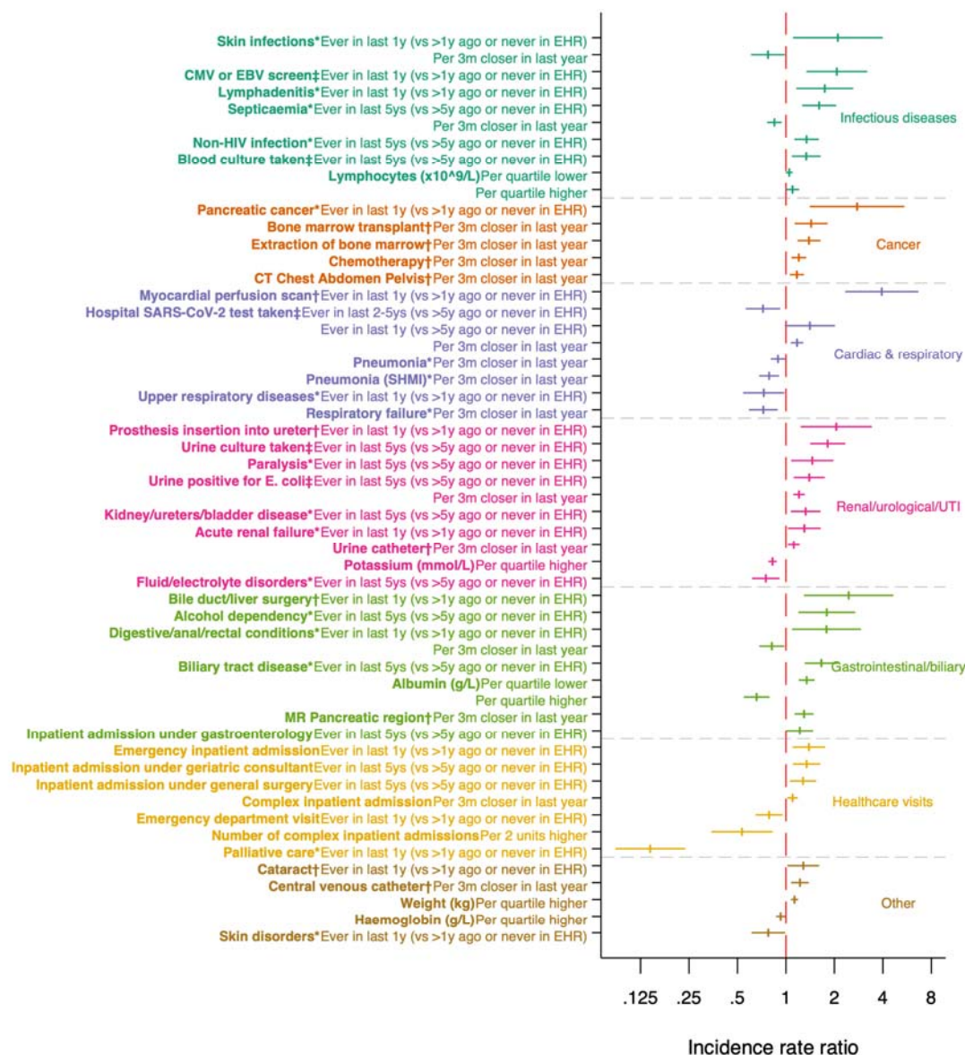
Figure 1: Adjusted associations (incidence rate ratios with 95% CIs) between selected characteristics and E. coli BSI risk in FY2022/23-2023/24.
