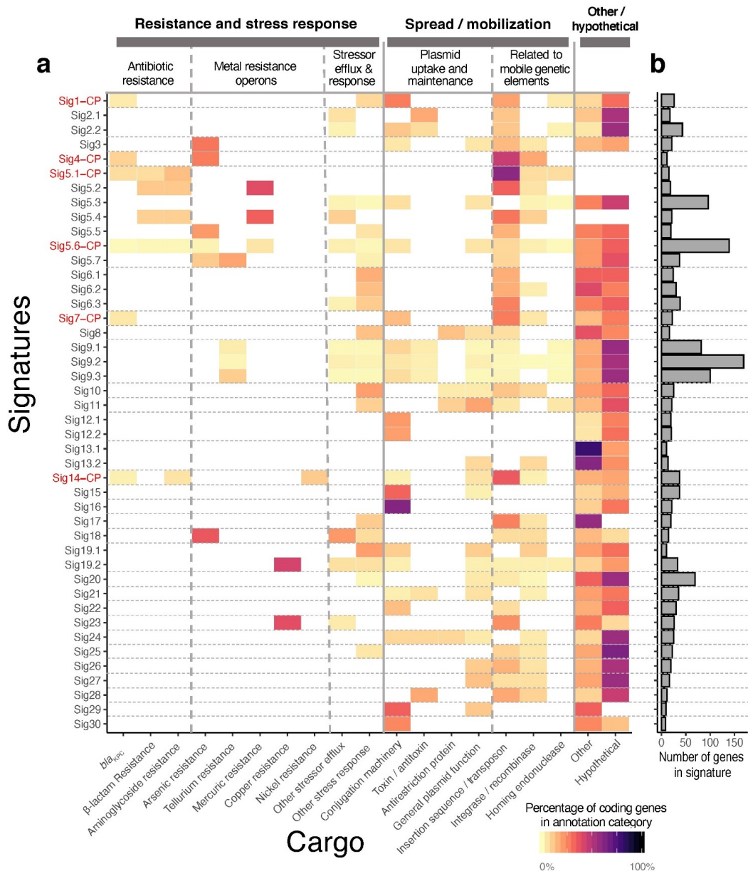
Figure S10. Signatures carried genes important for hospital adaptation and signature mobility. a, Each row in the heatmap corresponds to one of the 44 geographic signatures. Groups of signatures that nest into each other are separated by horizontal dashed lines. The predicted functions of 1,494 genes within our 44 signatures were categorized into five major functional categories, unless they fell outside of these categories (other) or no gene function could be predicted (hypothetical). The coloring of the heatmap indicates the percentage of genes of each signature that are assigned to a particular category. The identifiers of carbapenemase-carrying signatures are shown in red type and suffixed with -CP . b. Number of genes in each signature.
