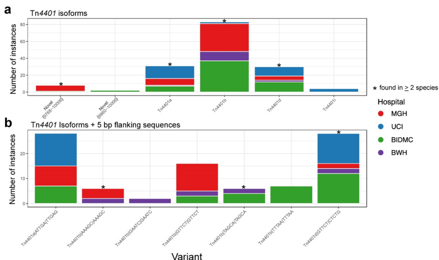
Figure S6: Limited tracing of carbapenemase localized spread using Tn4401 isoforms and their immediate flanking sequences. a , Number of instances for Tn4401 isoforms; and b , combinations of the three most common Tn4401 isoforms with their 5 bp flanking sequences which were found in multiple isolates from our study. Colors indicate the proportion of instances found in each of the four hospitals. The asterisk indicates forms that were found in multiple species.
