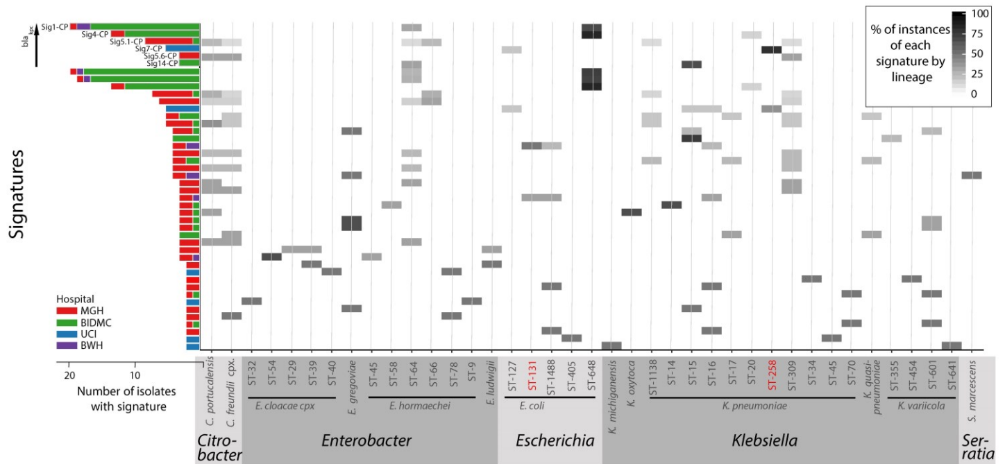
Figure S9. Signatures were present across diverse sequence types. In this heatmap, each row corresponds to a unique signature, and each column corresponds to a sequence type (ST). The shading represents the percentage of signature instances belonging to different taxonomic lineages, species or ST. The bar plot to the left of the heatmap depicts the number of isolates containing each signature, highlighting their prevalence across different hospitals.
