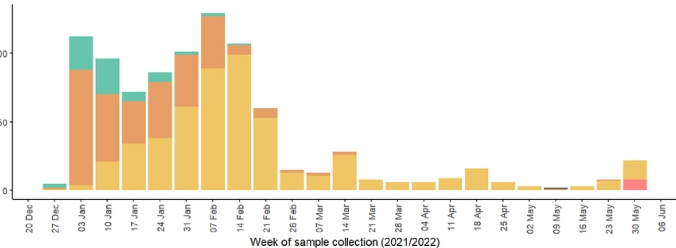
Figure 1. GISAID
