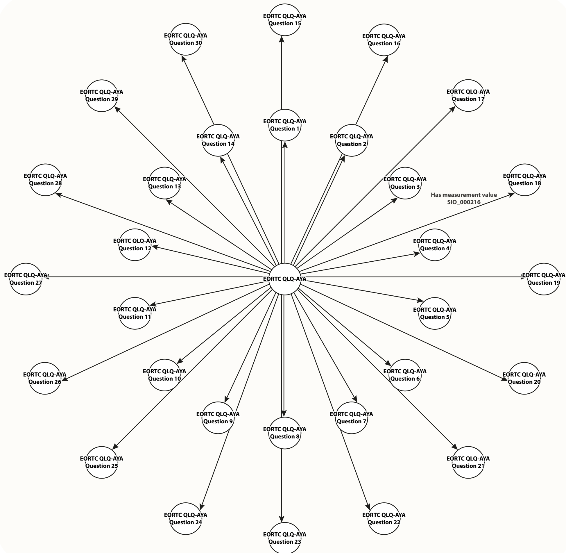
Supplementary Figure 2: Instrument graph illustrating the underlying measurements of a measurement instrument with multiple sub-concepts, such as here exemplified using the EORTC QLQ-AYA patient reported outcome measure.
