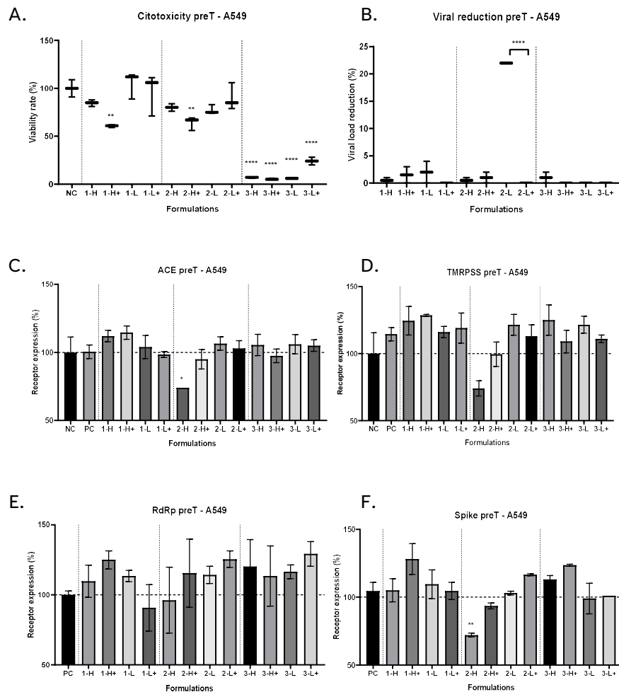
FIGURE 2.4 - A549 PRETREATMENT
