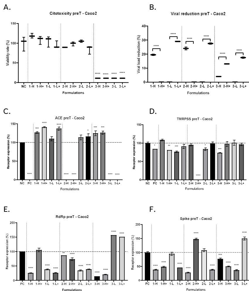
FIGURE 2.2 – CACO2 PRETREATMENT
