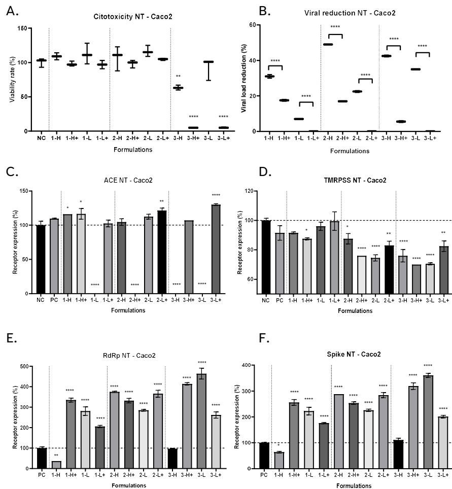
FIGURE 2.1 – CACO2 TREATMENT
