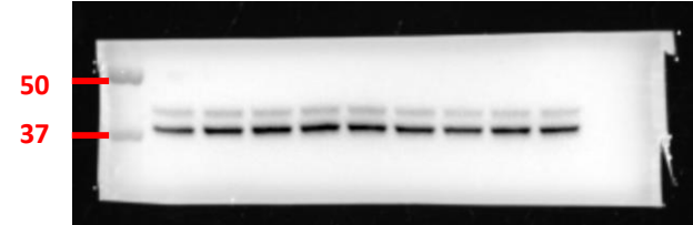
ERK Predicted MW 42-44 Kda
