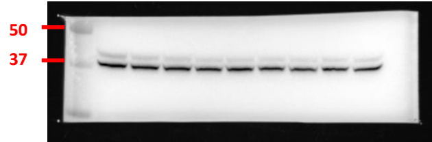
ERK Predicted MW 42-44 Kda
