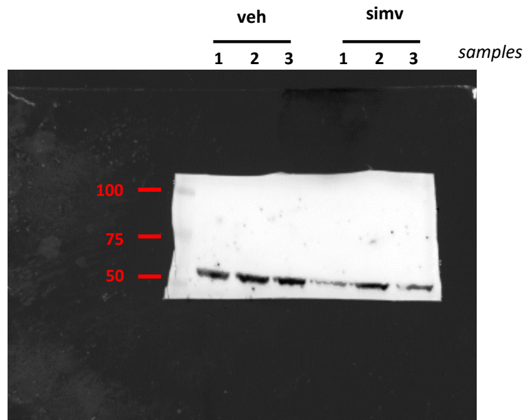
CB1 Predicted MW 53 Kda
