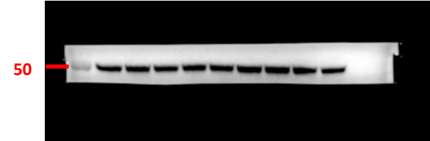
\alpha -tubulin predicted MW 50-55 Kda
