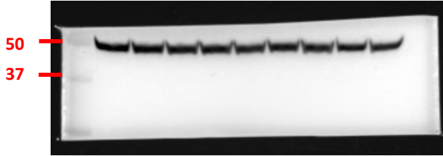
\alpha -tubulin predicted MW 50-55 Kda
