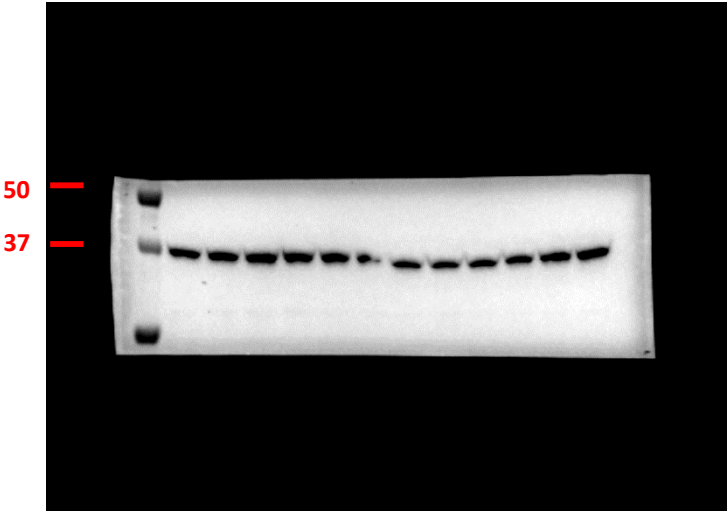
ERK Predicted MW 42-44 Kda
