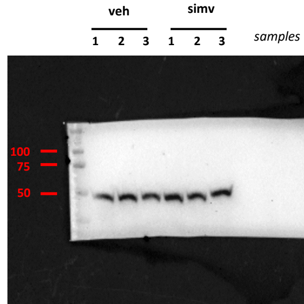
\alpha -tubulin predicted MW 50-55 Kda
