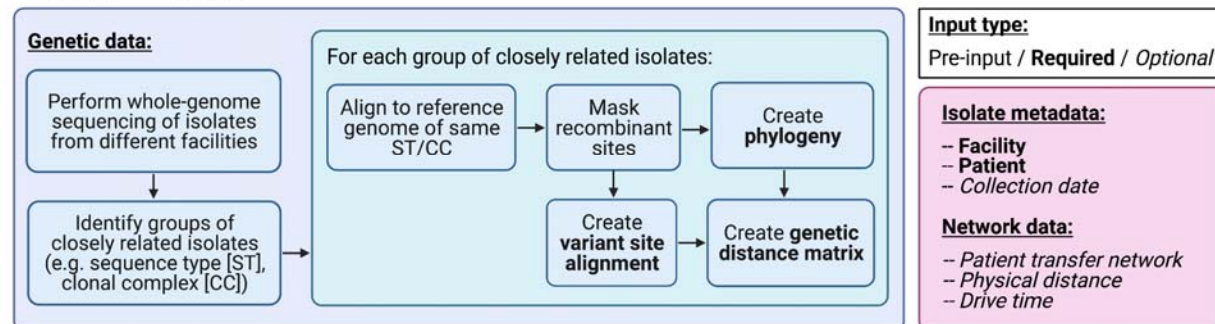
Figure 1: regentrans input data. Required and optional isolate genetic data and metadata for using regentrans. Figure created on BioRender.com.
