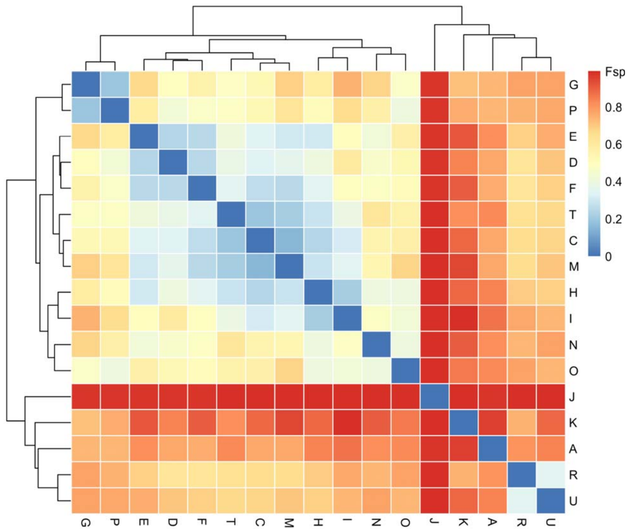
Figure 5: Some facility pairs have similar populations, indicating potential transmission between them. Genetic flow (Fsp) was calculated using the get_genetic_flow() function in regentran. Rows and columns are facilities. Lower Fsp indicates more similar populations and thus more putative transmission. At least two isolates are required from a facility to perform the Fsp calculation as within-facility variation must be calculated, so facilities with only one isolate have been removed. The heatmap is clustered based on Fsp values.
