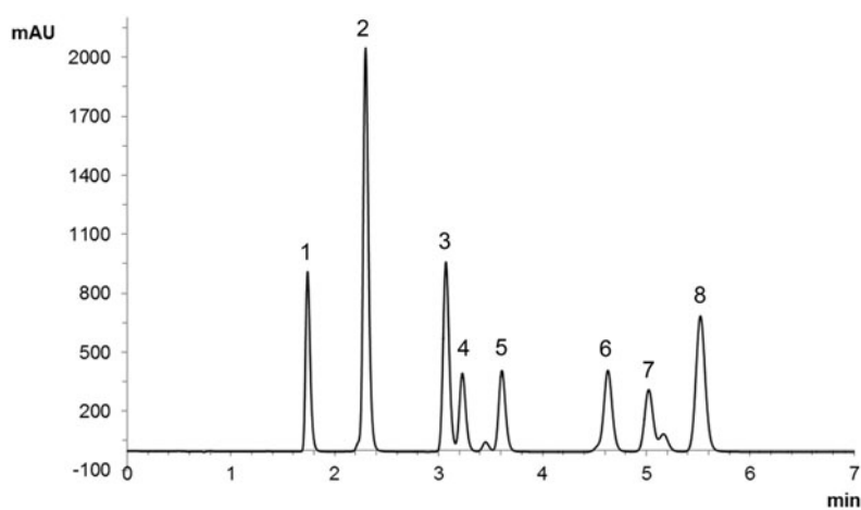
SUPPLEMENTARY FIG. S2. Sample chromatogram of a calibration standard. Formaldehyde-DNPH (1), acetaldehyde-DNPH (2), acetone-DNPH (3), acrolein-DNPH (4), propionaldehyde-DNPH (5), crotonaldehyde-DNPH (6), 2-butanone-DNPH (7), and butyraldehyde-DNPH (8).
