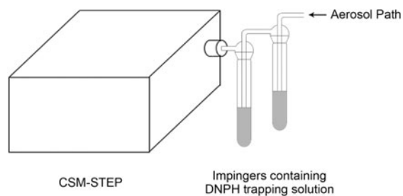
SUPPLEMENTARY FIG. S1. Schematic of carbonyl trapping apparatus. CSM, cigarette smoking machine; DNPH, 2,4-dinitrophenylhydrazine.
