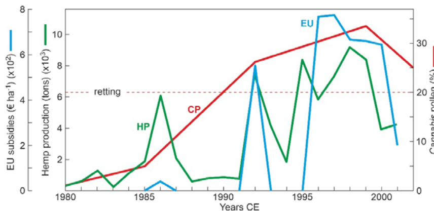
Figure 4. Hemp production in NE Spain (HP) and European Union subsidies to hemp cultivation (EU) (raw data from Gorchs & Lloberas, 2003) compared with the Cannabis pollen percentage curve from Lake Montcortès sediments (CP) (Fig. 2).
