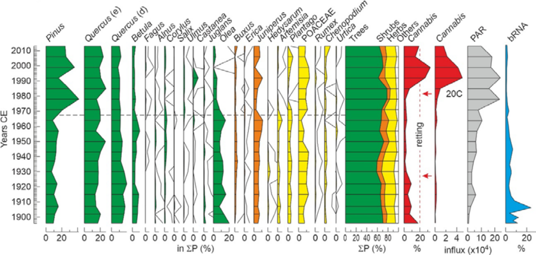
Figure 2. Percentage pollen diagram corresponding to the 20 th century at subdecadal (~5-year) resolution. Influx values (grains/particles cm -2 y -1 ) for Cannabis and pollen accumulation rates (PAR) are also provided. RNA from retting bacteria (bRNA) is represented in percentage with respect to the total bacterial flora (Rull et al., 2022). Solid lines are x10 exaggeration. Red arrows represent the major shifts in Cannabis pollen percentage. ΣP, pollen sum.
