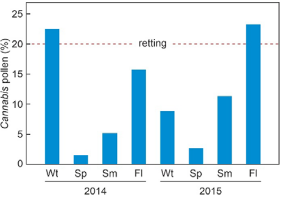
Figure 3. Seasonal distribution of sedimentary Cannabis pollen in Lake Montcortès during 2014 and 2015 (Rull et al., 2017). The hemp retting threshold (20%) is indicated by a red dashed line. Wt, winter; Sp, spring; Sm, summer; FI, fall.
