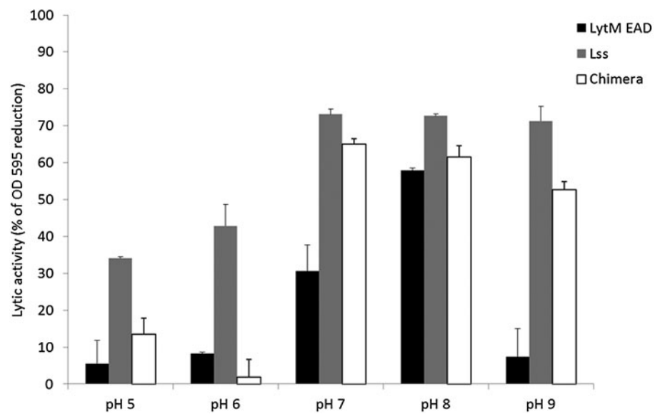
SUPPLEMENTARY FIG. S2. Enzyme activities in various pH conditions observed as a turbidity reduction after 1 hr at room temperature.
