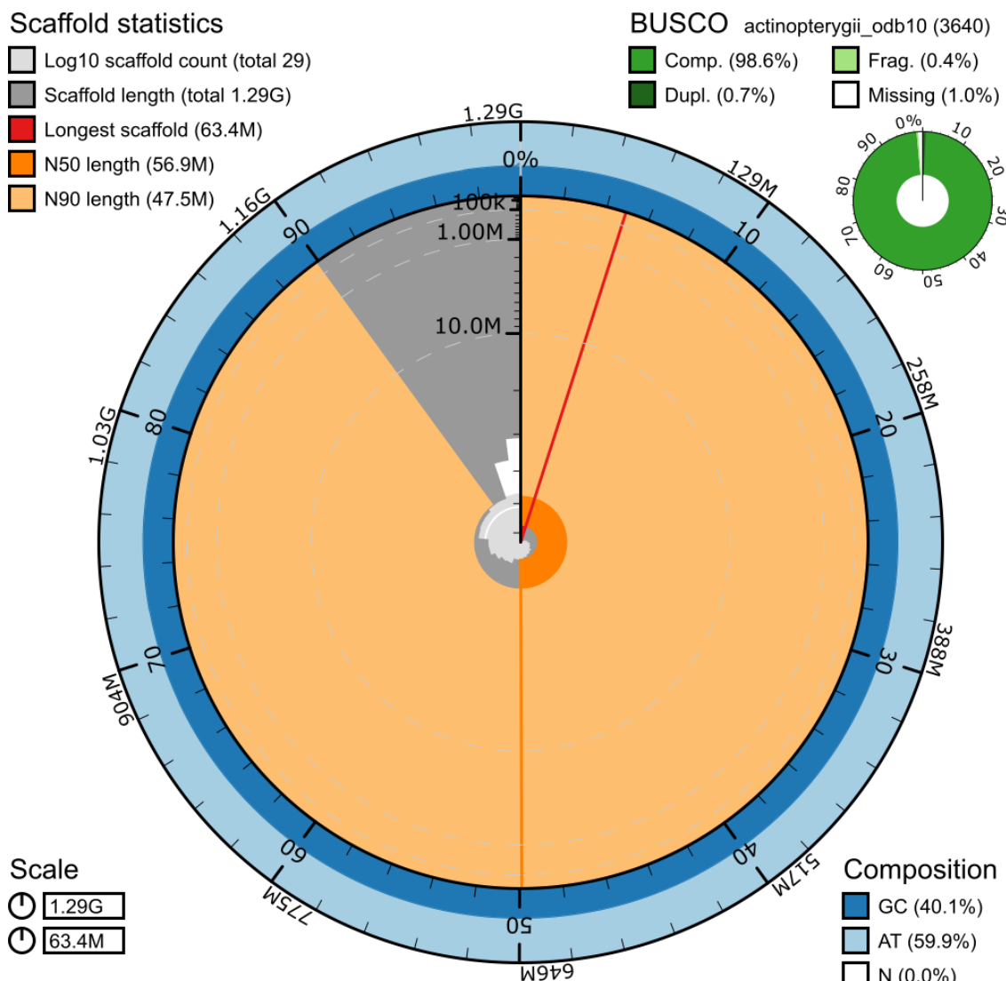
Figure 1. Snail plot summary of assembly statistics. The main plot is divided into 1,000 size-ordered bins around the circumference, with each bin representing 0.1% of the 1,291,697,043 bp assembly including the mitochondrial genome. The distribution of sequence lengths is shown in dark grey, with the plot radius scaled to the longest sequence present in the assembly (63,361,188 bp, shown in red). Orange and pale-orange arcs show the scaffold N50 and N90 sequence lengths (56,937,854 and 47,505,306 bp), respectively. The pale grey spiral shows the cumulative sequence count on a log-scale, with white scale lines showing successive orders of magnitude. The blue and pale-blue area around the outside of the plot shows the distribution of GC, AT, and N percentages in the same bins as the inner plot. A summary of complete, fragmented, duplicated, and missing BUSCO genes found in the assembled genome from the Actinopterygii database (odb10) is shown in the top right.
