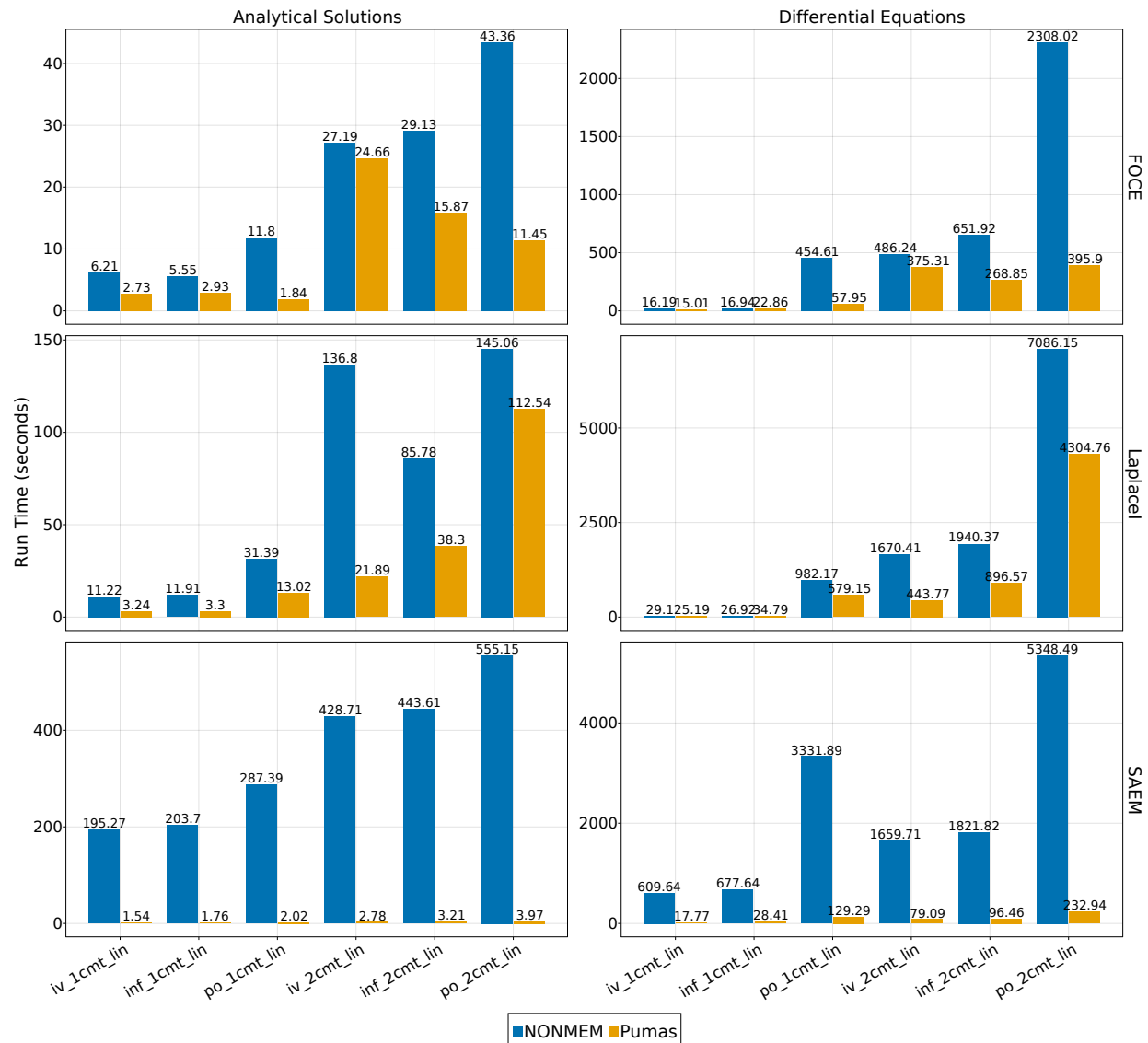
Figure 10: Maximum likelihood estimation and SAEM benchmark results for multiple dosing simulations.. Shown is the run time of a fit of the various Pk/Pd models with the FOCE, LaplaceI, and SAEM population integral approximation schemes in NONMEM and Pumas. Analytical solutions refers to direct usage of the solution to the differential equation in the fitting process. For numerical approximations, NONMEM was run using ADVAN6 (the DVERK 6th order Runge-Kutta method) while Pumas used the Vern7 ODE solver.
