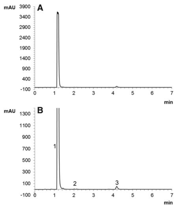
SUPPLEMENTARY FIG. S5. Full (A) and enhanced (B) chromatograms for a sample blank. Unreacted DNPH (1), trace formaldehyde-DNPH (2), and acetone (2). Peak identities were confirmed with additional spiking.
