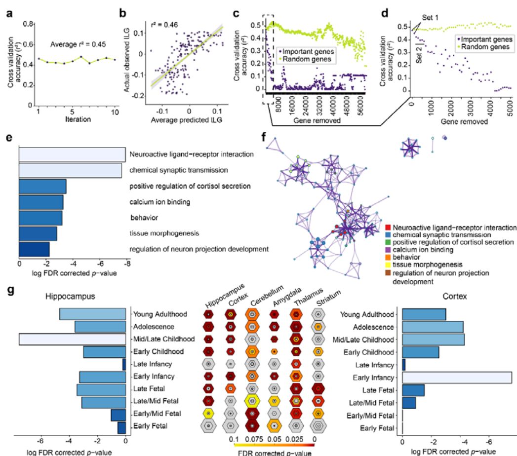
Figure 5 | Transcriptomic association analysis of the hippocampal ILG. a, Accuracy ( r^2 ) for ten separate 10-fold cross-validated LASSO-PCR models for ILG prediction using normalized gene expression data provided by the Allen Human Brain Atlas. b, Relationship between the average predicted ILG for the aforementioned ten separate 10-fold cross-validated models and the actual observed ILG. c, Systematic removal of the top 100 critical probes identified by our prediction model was undertaken. Following each removal, the 10-fold cross-validation accuracy in predicting ILG values was documented (purple dots). To establish a comparative baseline, an iterative process involving the removal of 100 random probes was also executed (chartreuse). d, In the zoomed-in view of panel c , we scrutinized the initial 50 rounds of 100-probe removal. Notably, a significant decline in performance became evident and this decline was not recovered following the removal of 200 and 700 genes. e, A bar graph depicts the enriched biological pathways
