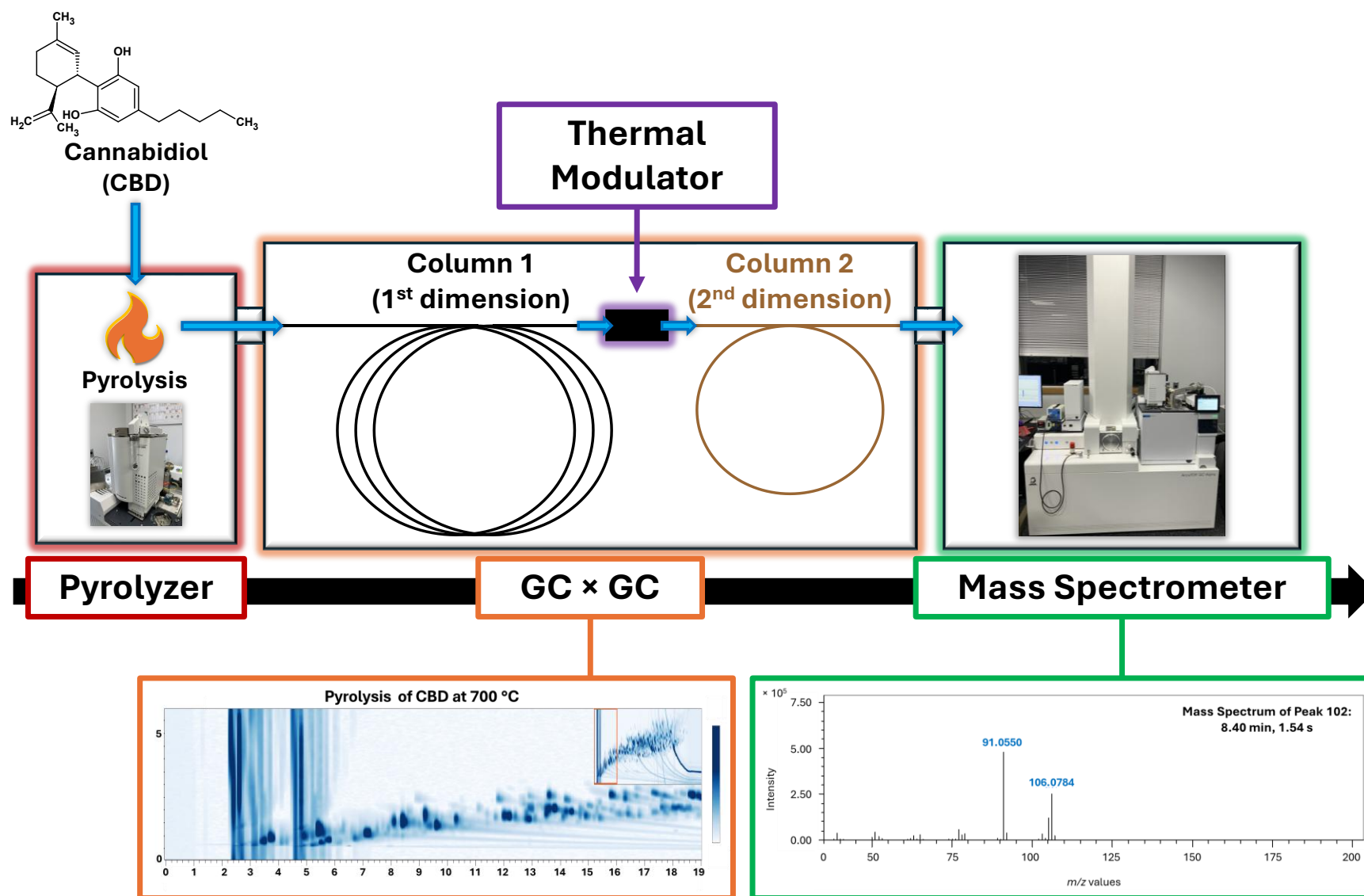
Figure S1. Schematic of the instrument set up used for the pyrolysis and GC × GC – HRMS analysis of CBD.
