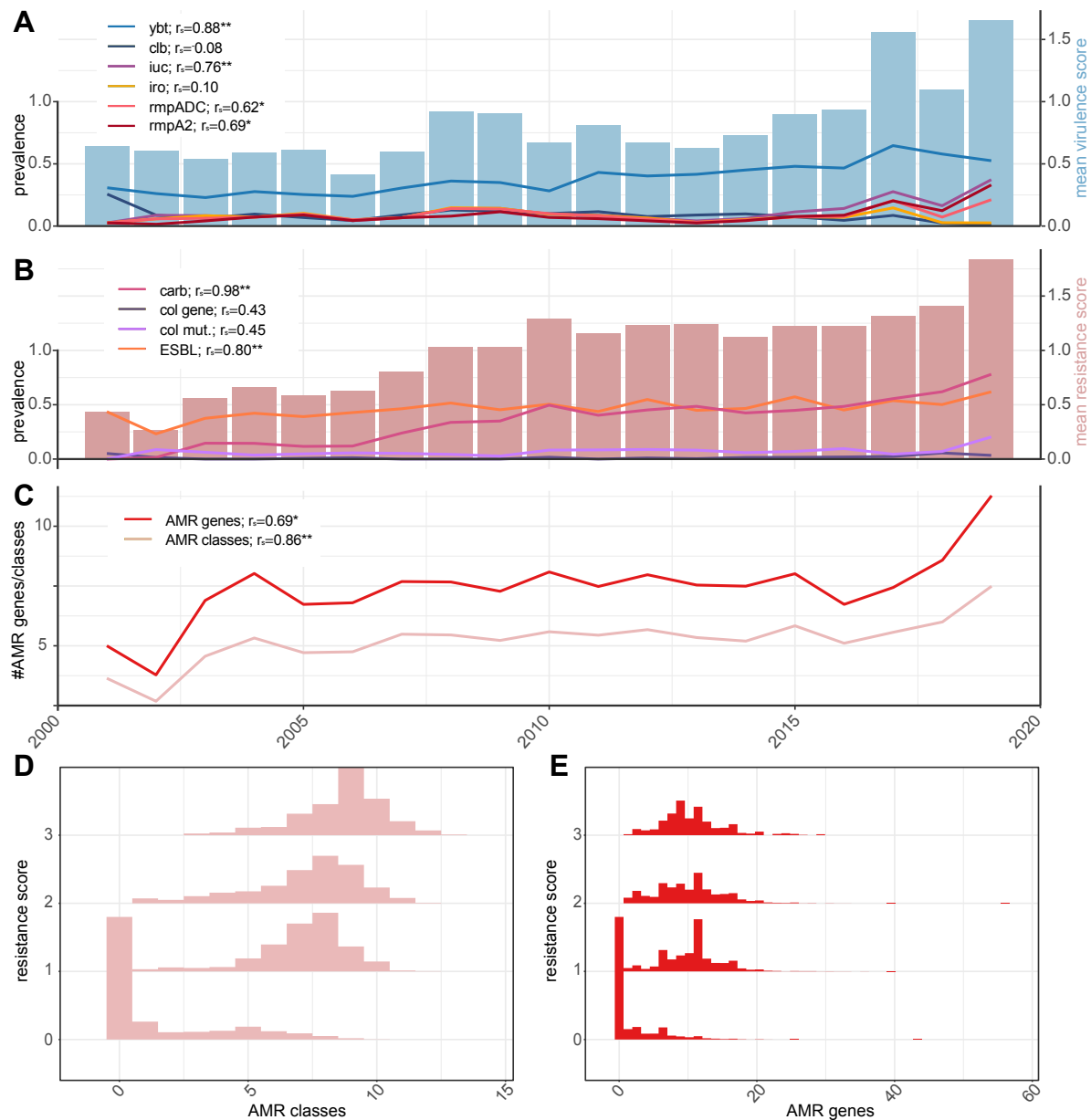
Figure 1. Relationships between Kleborate virulence and resistance scores and the prevalence of key virulence and antimicrobial resistance (AMR). Data shown summarise Kleborate results for non-redundant set of 9,705 publicly available K. pneumoniae genomes (Table S2). (A) Mean virulence score (barplot, right y-axis) and prevalence of individual virulence loci (line plots, left y-axis) over time. Ybt, yersiniabactin; clb, colibactin; iuc, aerobactin; iro, salmochelin; rmpADC, hypermucoidy rmp locus; rmpA2, rmpA2 gene. Correlations between mean virulence score and prevalence of each locus are noted. (B) Mean resistance score (barplot, right y-axis) and prevalence of carbapenemases (carb), acquired colistin resistance genes (col gene), mutations in MgrB/PmrB (col mut) and genes conferring resistance to extended-spectrum \beta -lactams (ESBL) (line plots, left y-axis).
