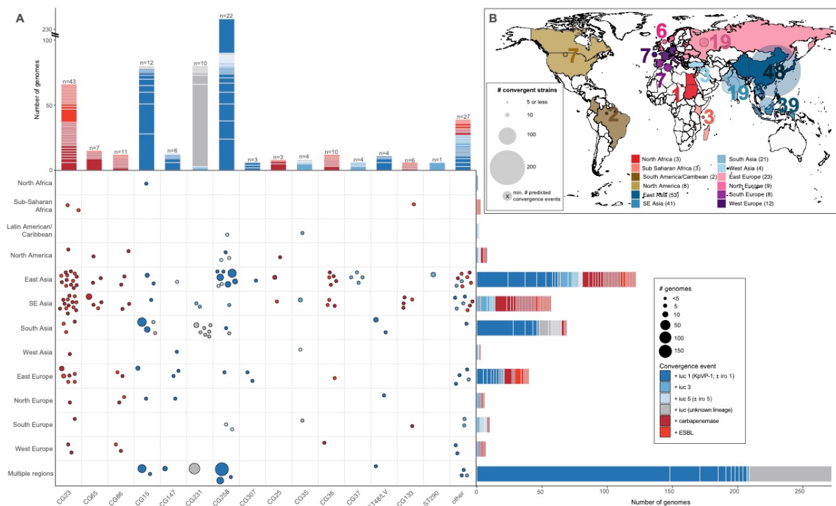
Figure 7. Convergence of AMR and virulence determinants in the K. pneumoniae population, identified by Kleborate analysis of public genomes. (A) Geographical and lineage distribution of convergence events. Each circle represents a unique convergence event (i.e. a monophyletic clade harbouring both ESBL/carbapenemase genes and iuc ; see interactive tree at https://microreact.org/project/JDyan46yctyDh6weEUjWN , summary of events in Table S8 , assignment of genomes to events in Table S2 ). Circles are scaled by the number of total genomes linked to the event and colored to indicate whether convergence is inferred to have occurred via acquisition of AMR gene/s (ESBL or carbapenemase/s) by a hypervirulent lineage or via acquisition of an iuc -encoding plasmid by an AMR lineage, as per inset legend. Marginal barplots show the number of convergence events (color blocks) and genomes (block heights) associated with each lineage (top) or geographical region (right). Lineages were defined on the basis of multi-locus sequence types (STs), number of convergence events estimated for each is labelled at the top of each bar. (B) Distribution of convergent genomes by location. Countries from which convergent genomes were detected are colored on the map; circles represent the number of convergent genomes detected in each UN-defined geographical region (indicated by color, as per inset legend), scaled and labelled
